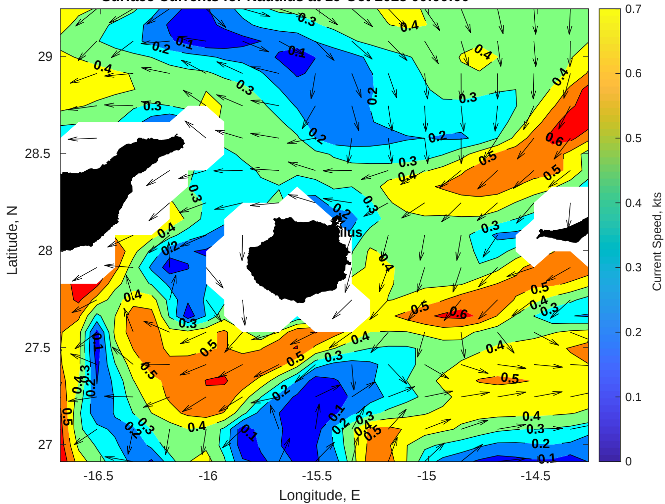
Surface Currents for Nautilus at 19-Oct-2025 00:00:00
