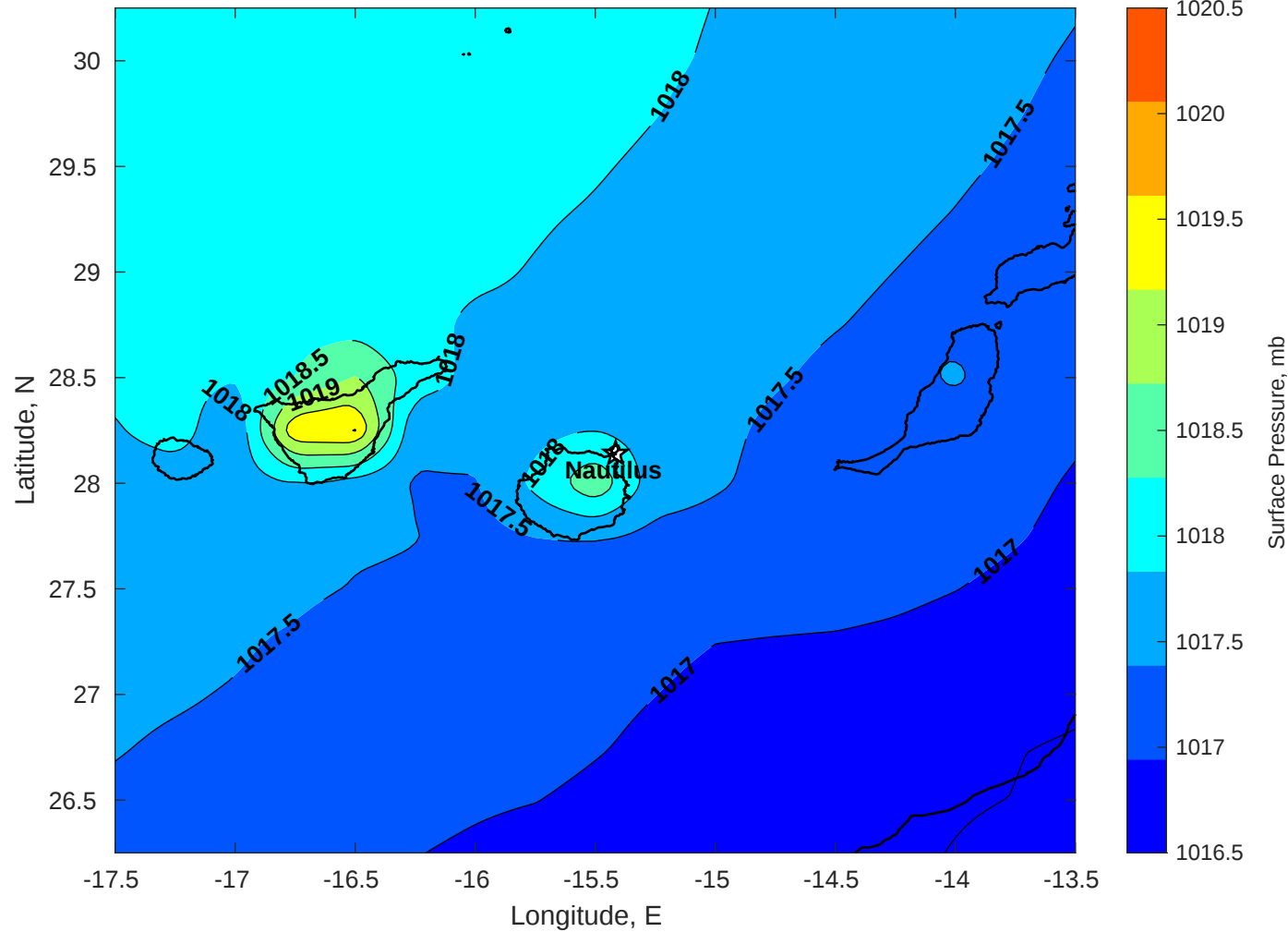
Surface Pressure (mb) for Nautilus at 21-Oct-2025 00:00:00
