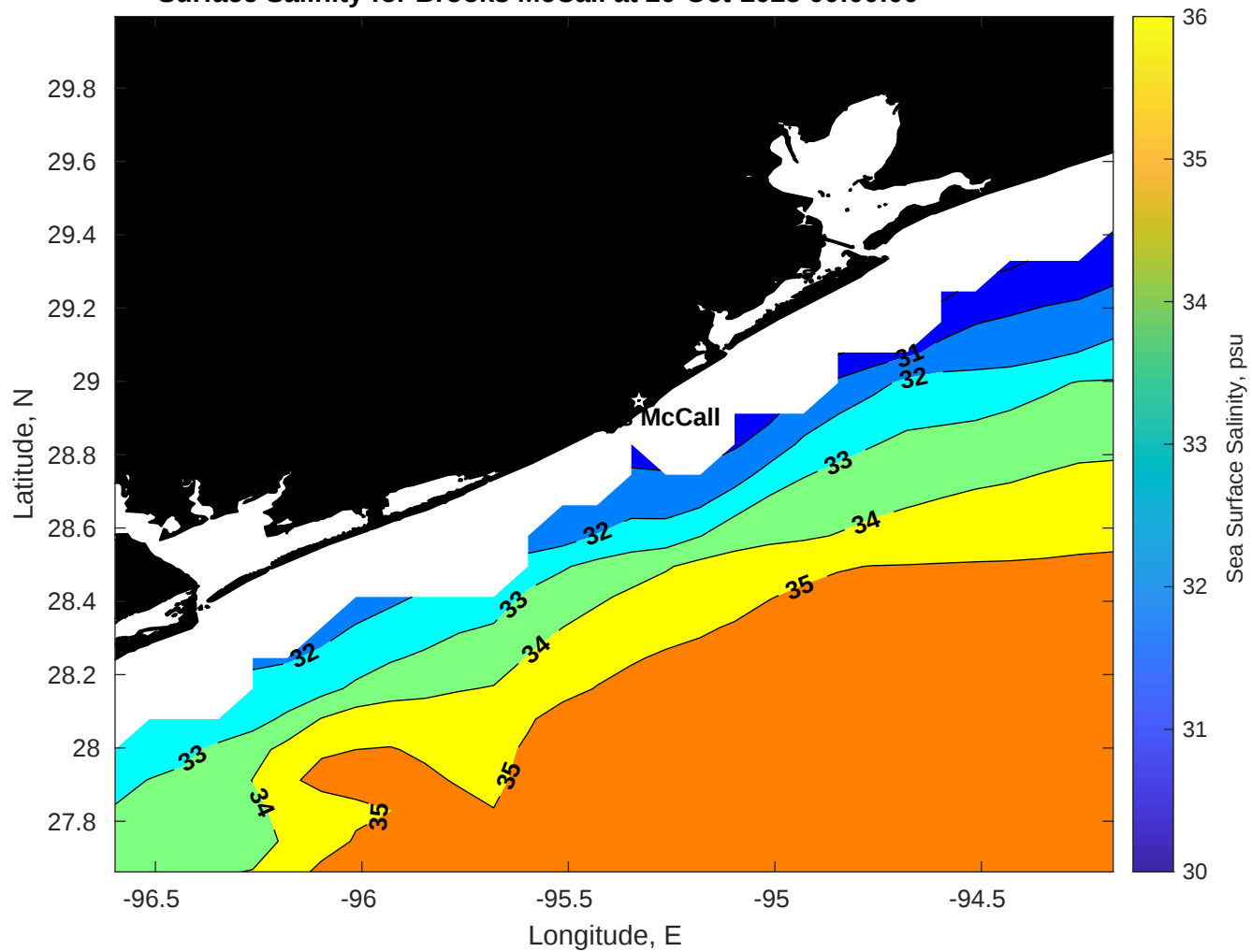
Surface Salinity for Brooks McCall at 20-Oct-2025 00:00:00
