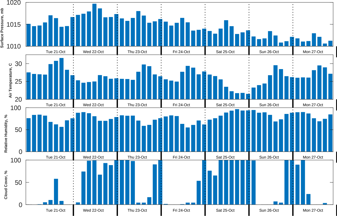
Met Forecast for Brooks McCall from 21-Oct-2025 00:00:00 to 28-Oct-2025 00:00:00
