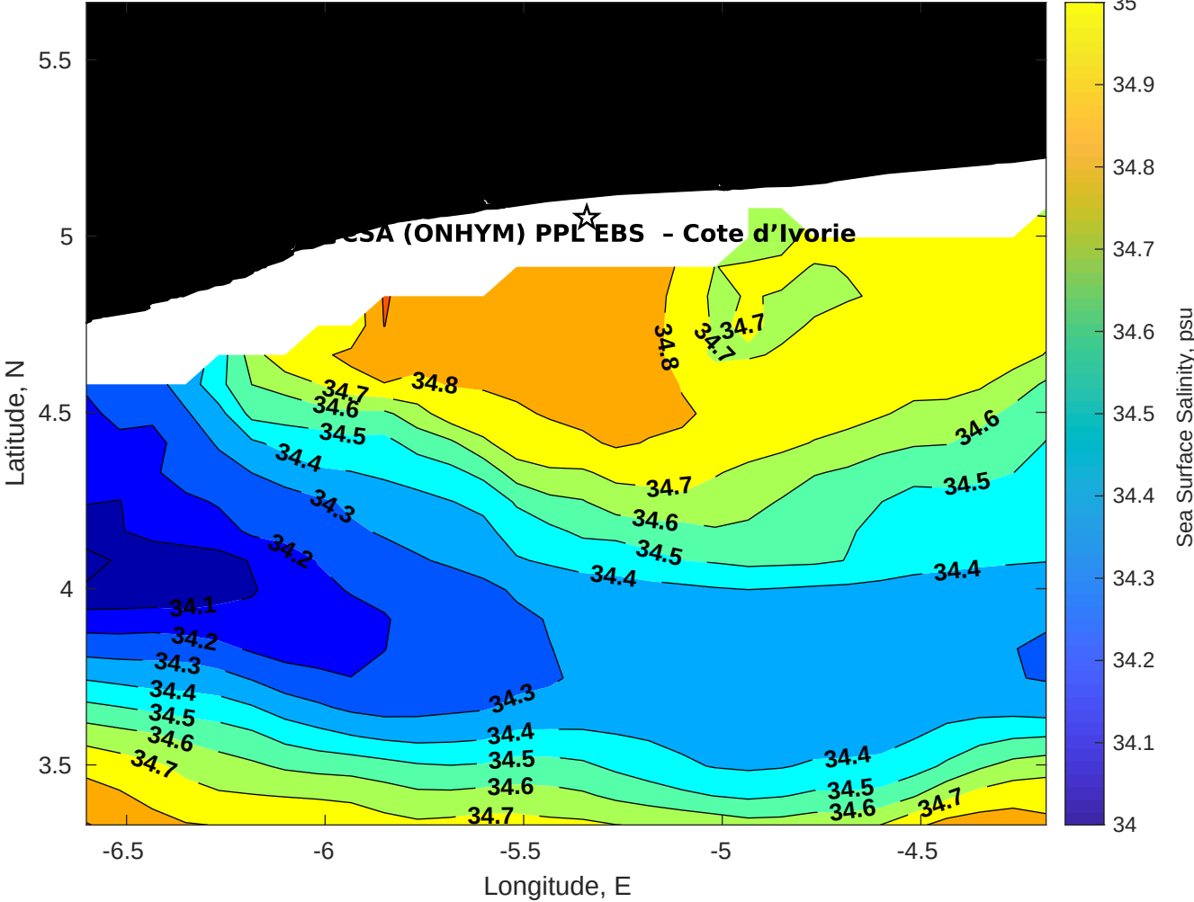
Surface Salinity for CSA (ONHYM) PPL EBS - Cote d'Ivoire at 20-Oct-2025 00:00:00
