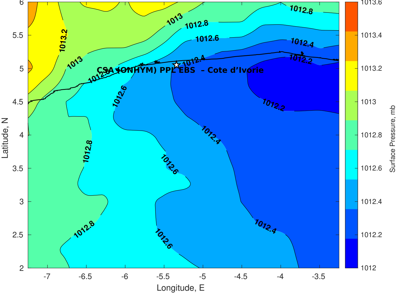
Surface Pressure (mb) for CSA (ONHYM) PPL EBS - Cote d'Ivoire at 21-Oct-2025 00:00:00
