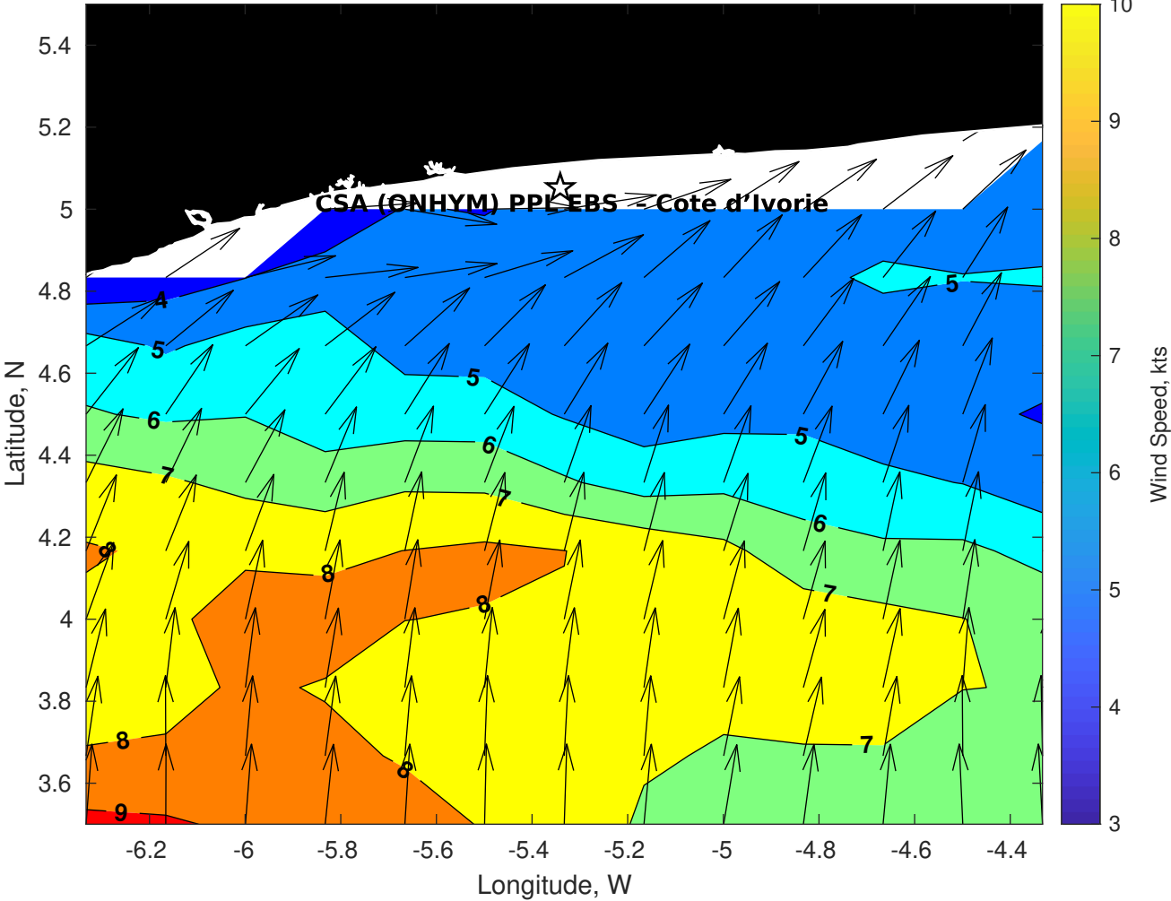
Winds (kts) for CSA (ONHYM) PPL EBS - Cote d'Ivoire at 21-Oct-2025 09:00:00
