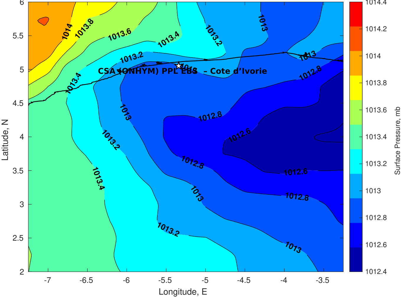
Surface Pressure (mb) for CSA (ONHYM) PPL EBS - Cote d'Ivoire at 22-Oct-2025 00:00:00
