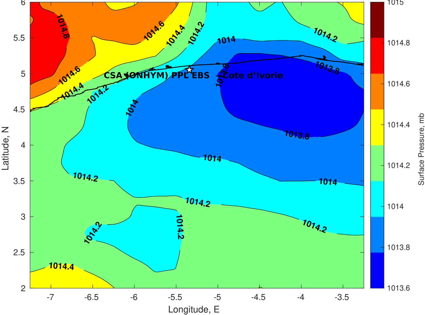
Surface Pressure (mb) for CSA (ONHYM) PPL EBS - Cote d'Ivoire at 23-Oct-2025 00:00:00
