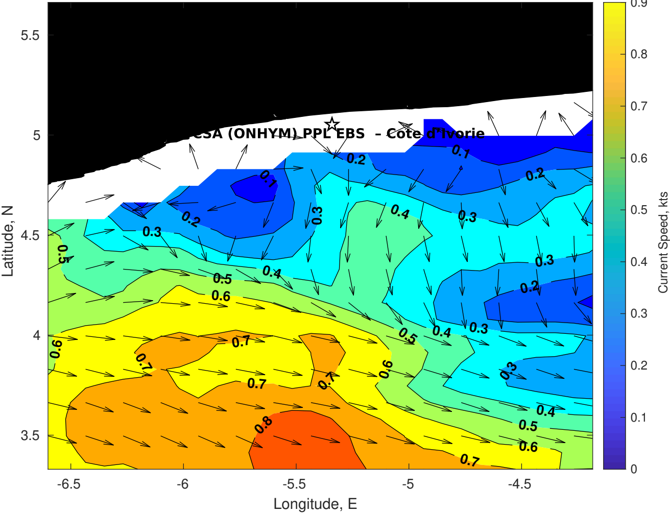
Surface Currents for CSA (ONHYM) PPL EBS - Cote d'Ivoire at 20-Oct-2025 00:00:00
