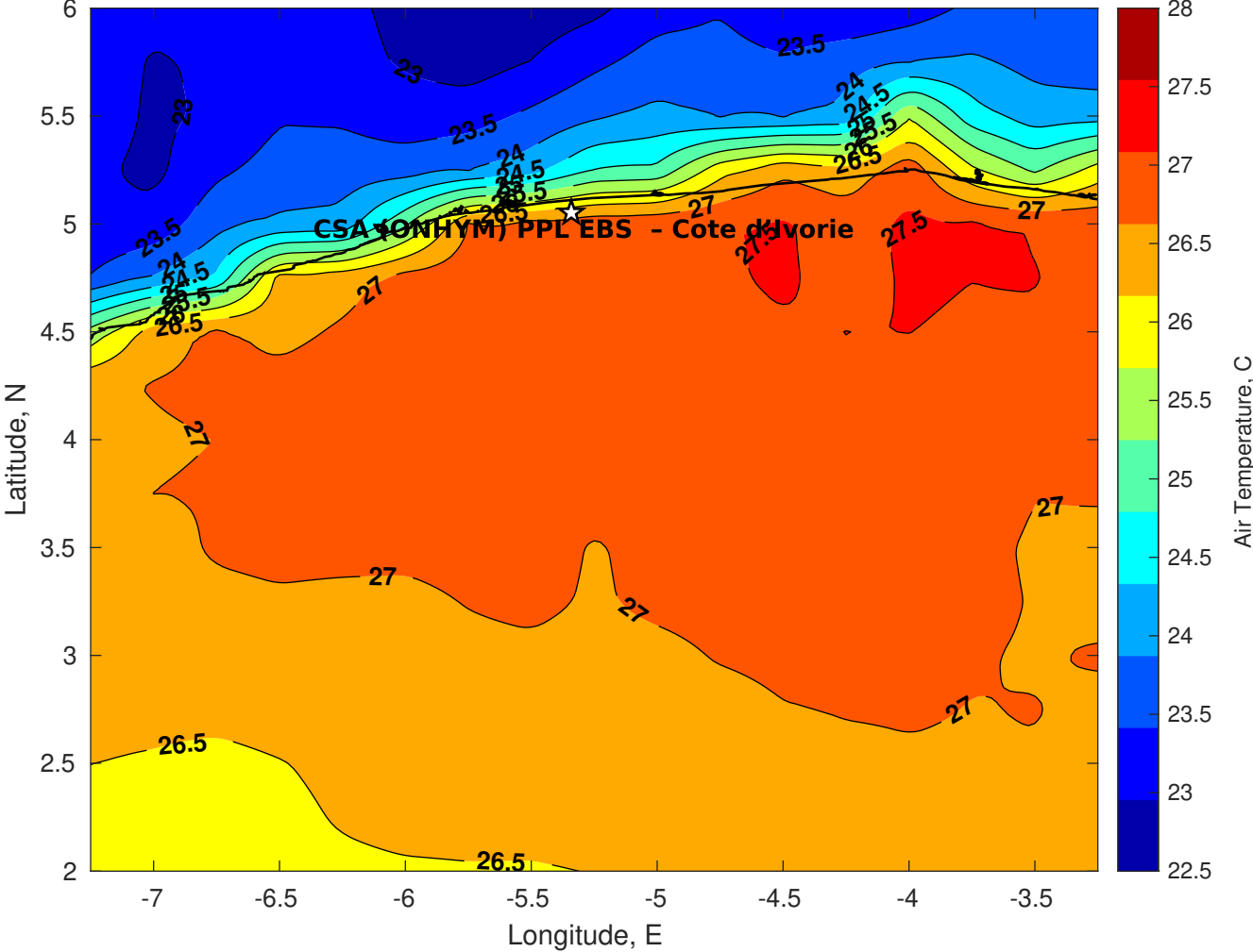
Air Temperature (C) for CSA (ONHYM) PPL EBS - Cote d'Ivoire at 21-Oct-2025
