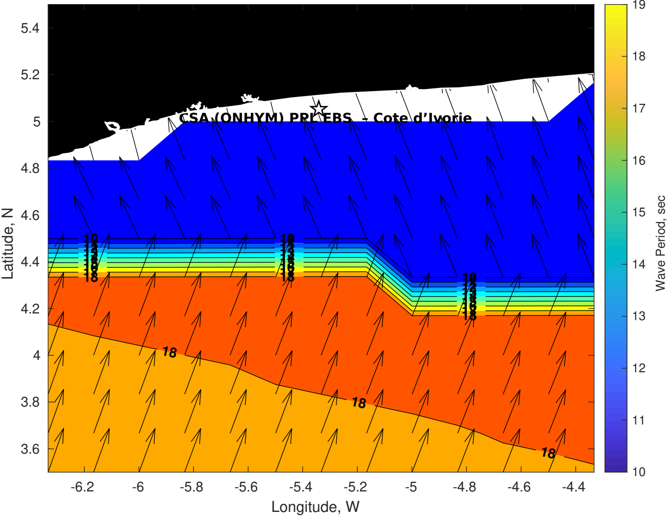
Wave Period (sec) for CSA (ONHYM) PPL EBS - Cote d'Ivoire at 21-Oct-2025 09:00:00
