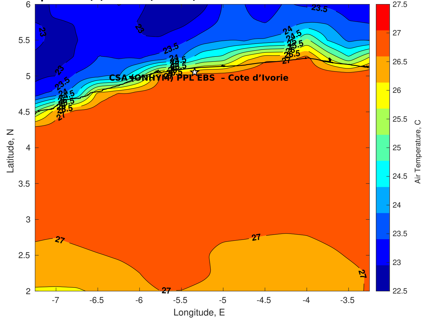
Air Temperature (C) for CSA (ONHYM) PPL EBS - Cote d'Ivoire at 21-Oct-2025
