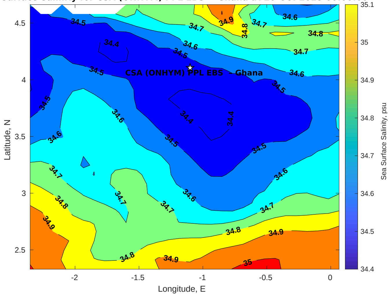
Surface Salinity for CSA (ONHYM) PPL EBS - Ghana at 20-Oct-2025 00:00:00
