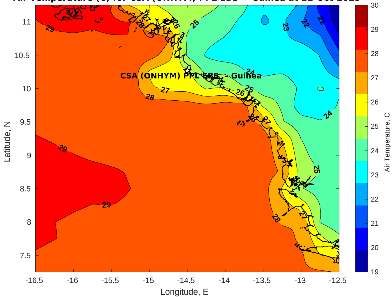
Air Temperature (C) for CSA (ONHYM) PPL EBS - Guinea at 21-Oct-2025
