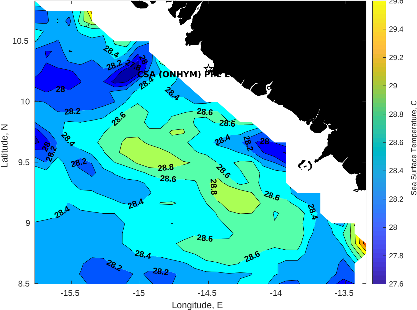
SST for CSA (ONHYM) PPL EBS - Guinea at 20-Oct-2025 00:00:00
