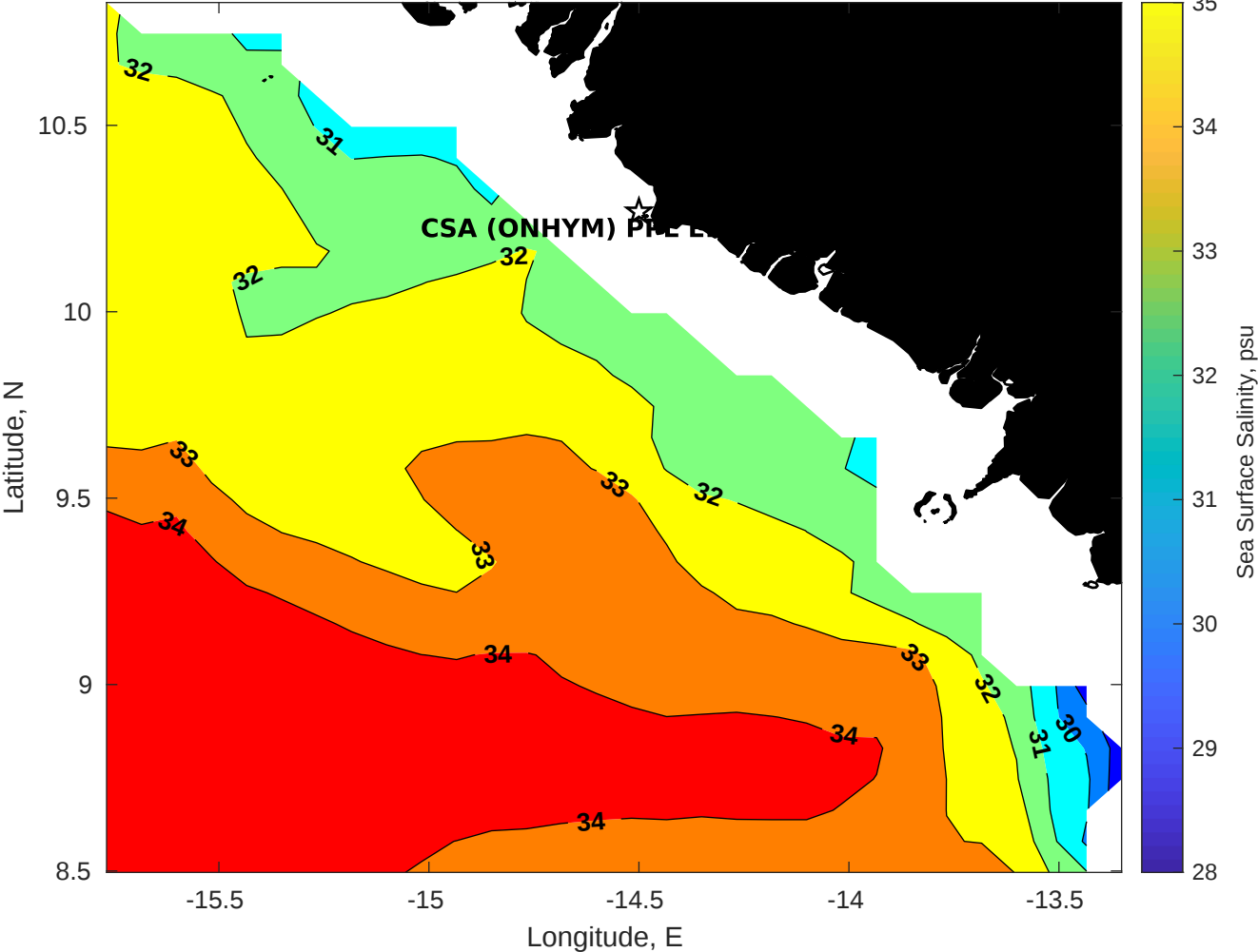
Surface Salinity for CSA (ONHYM) PPL EBS - Guinea at 20-Oct-2025 00:00:00
