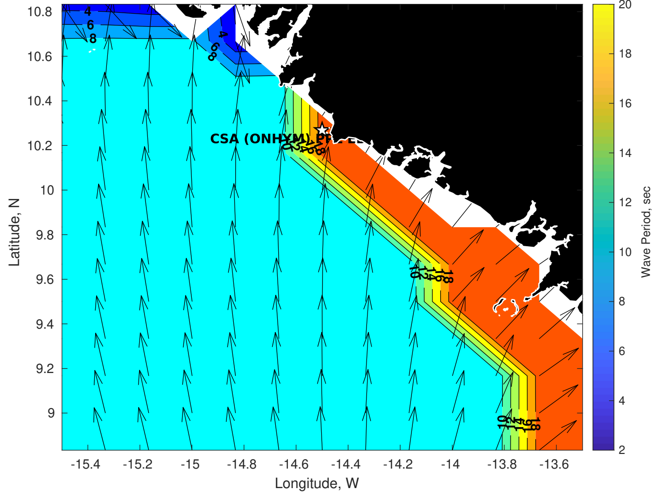
Wave Period (sec) for CSA (ONHYM) PPL EBS - Guinea at 21-Oct-2025 09:00:00
