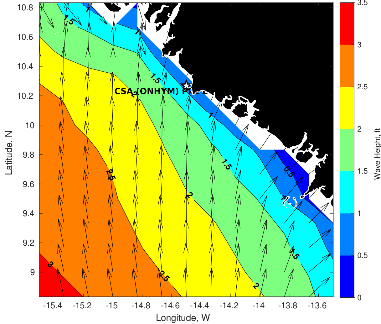
Wave Height (ft) for CSA (ONHYM) PPL EBS - Guinea at 21-Oct-2025 09:00:00
