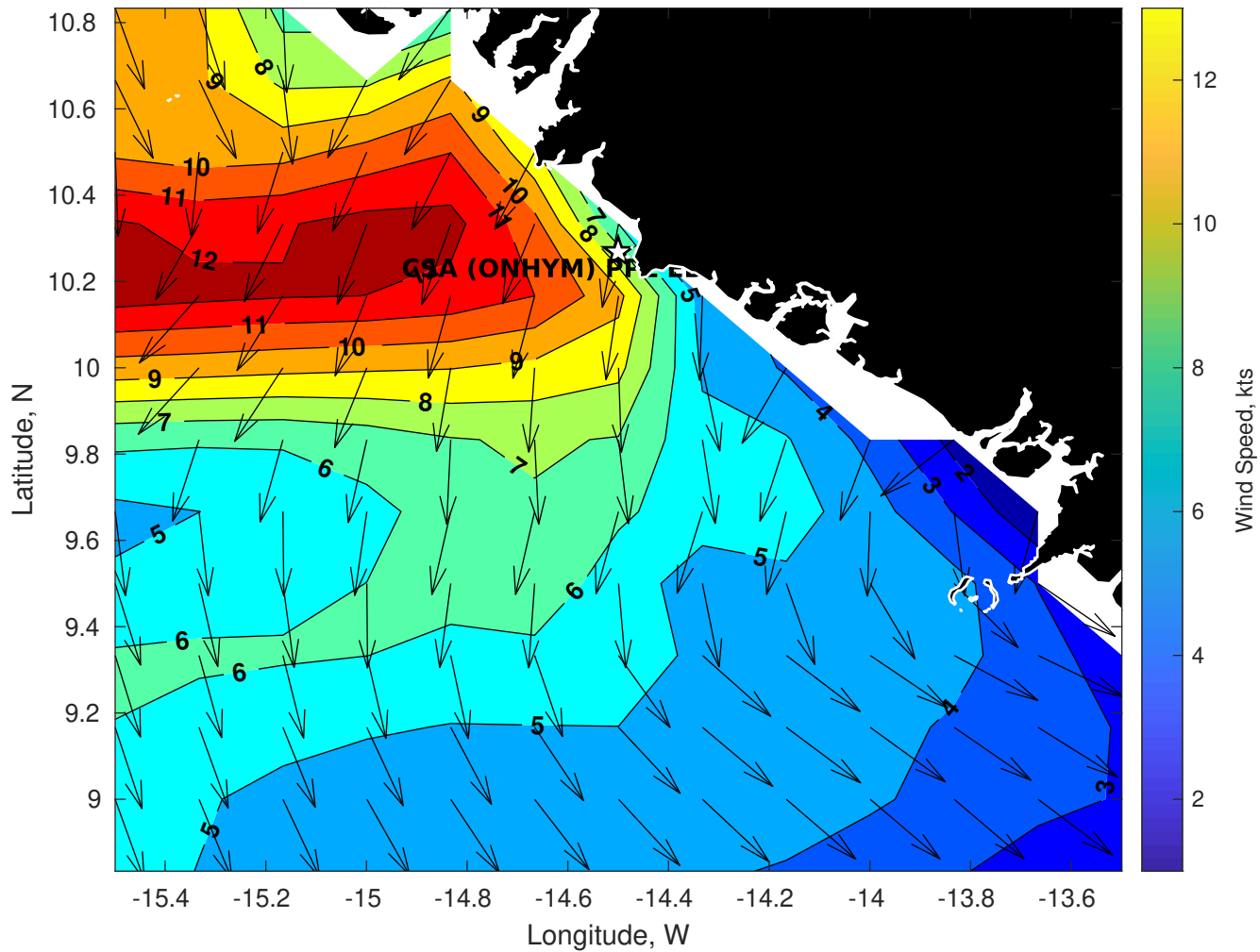
Winds (kts) for CSA (ONHYM) PPL EBS - Guinea at 21-Oct-2025 09:00:00
