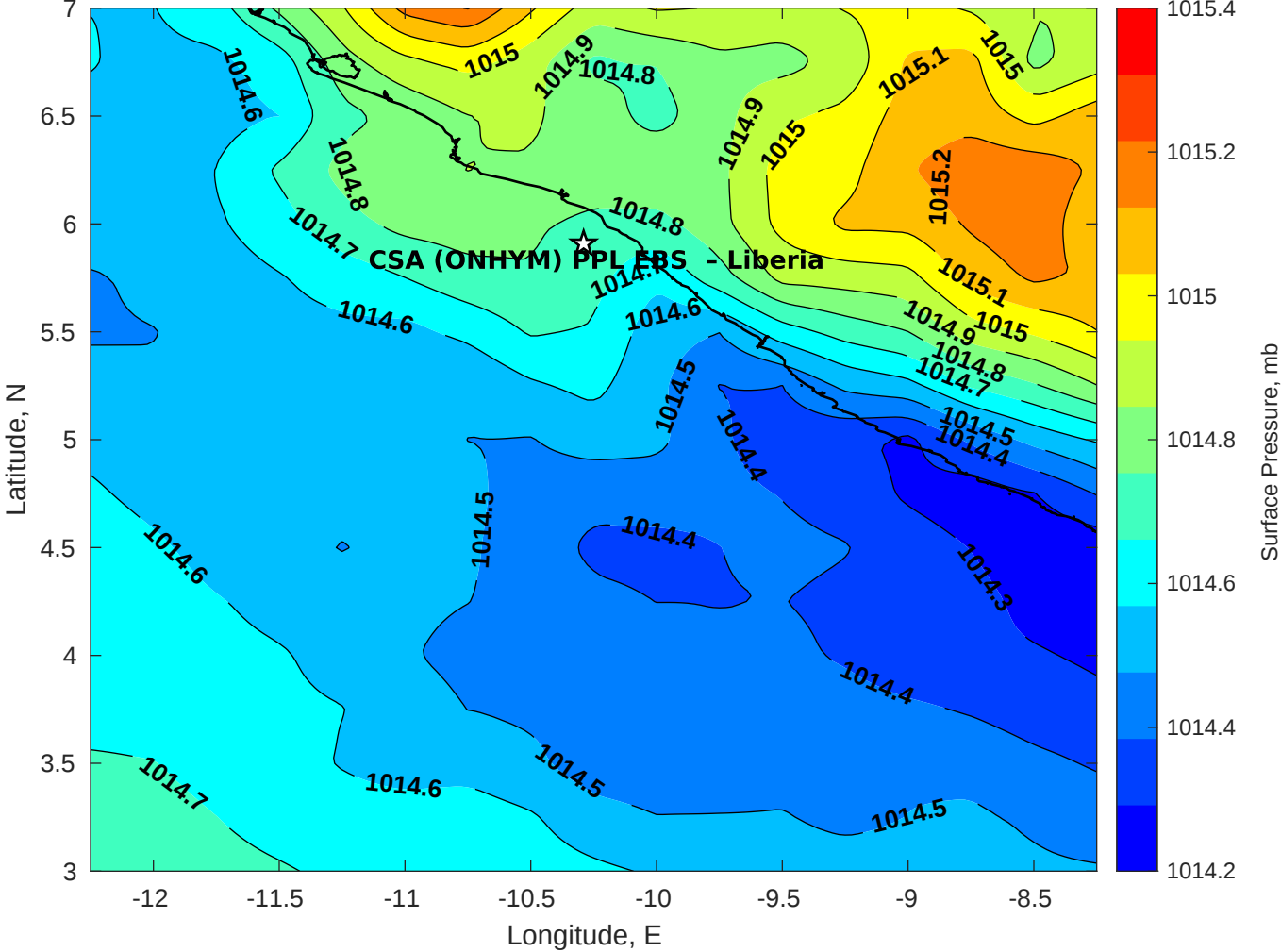
Surface Pressure (mb) for CSA (ONHYM) PPL EBS - Liberia at 23-Oct-2025 00:00:00
