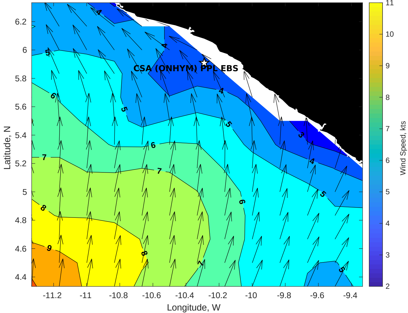
Winds (kts) for CSA (ONHYM) PPL EBS - Liberia at 21-Oct-2025 09:00:00
