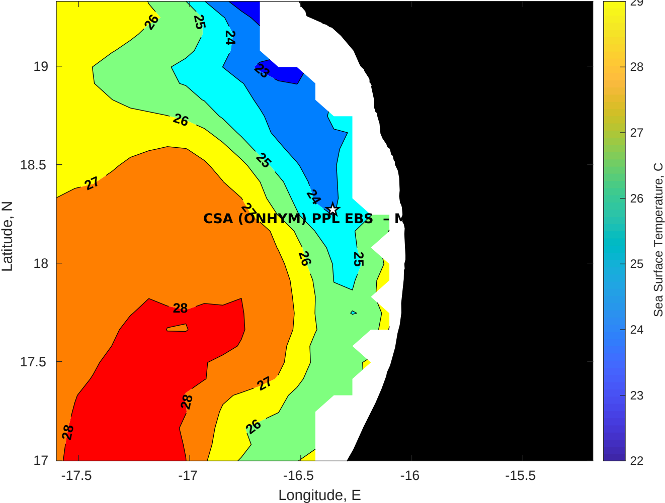
SST for CSA (ONHYM) PPL EBS - Mauritania at 20-Oct-2025 00:00:00
