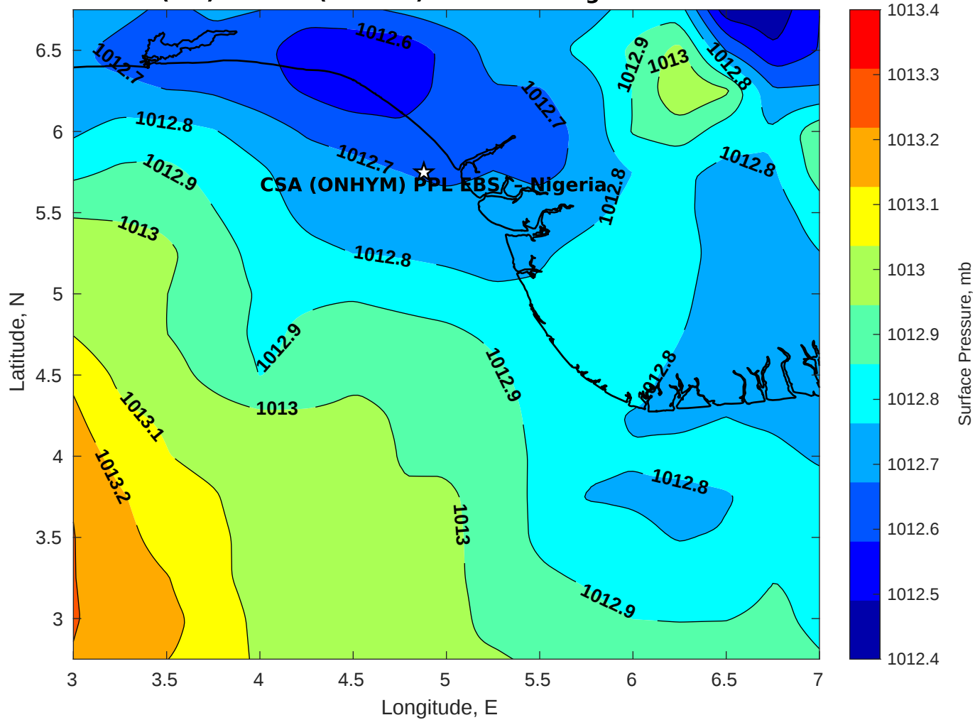
Surface Pressure (mb) for CSA (ONHYM) PPL EBS - Nigeria at 23-Oct-2025 00:00:00
