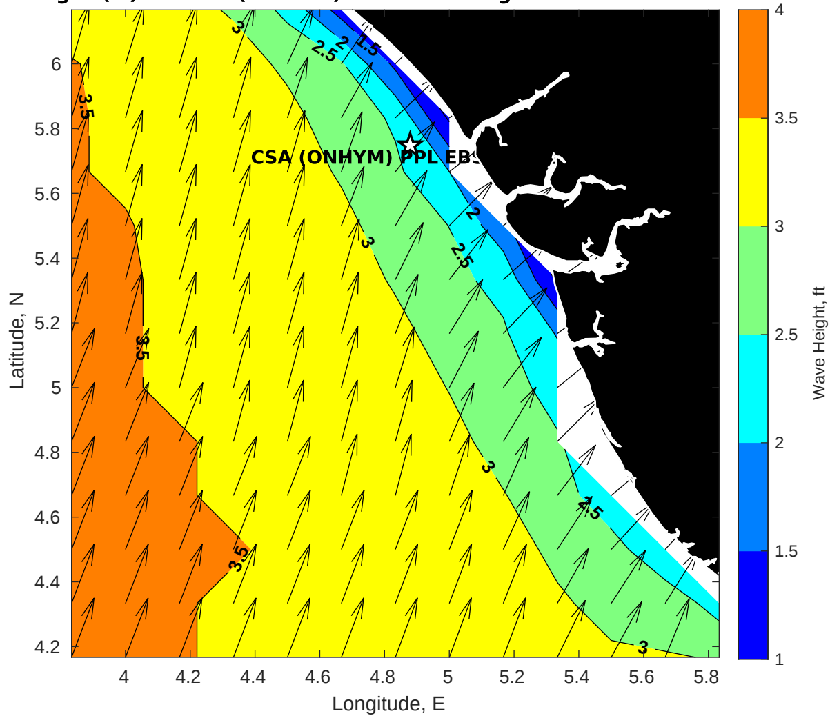
Wave Height (ft) for CSA (ONHYM) PPL EBS - Nigeria at 21-Oct-2025 09:00:00
