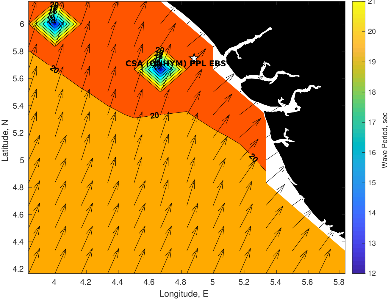
Wave Period (sec) for CSA (ONHYM) PPL EBS - Nigeria at 21-Oct-2025 09:00:00
