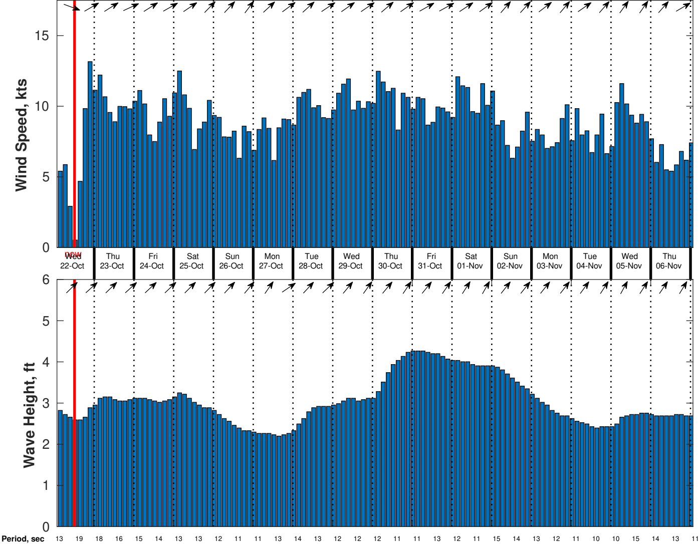
Wind & Wave Forecast for CSA (ONHYM) PPL EBS - Nigeria from 21-Oct-2025 02:00:00 to 06-Nov-2025 02:00:00
