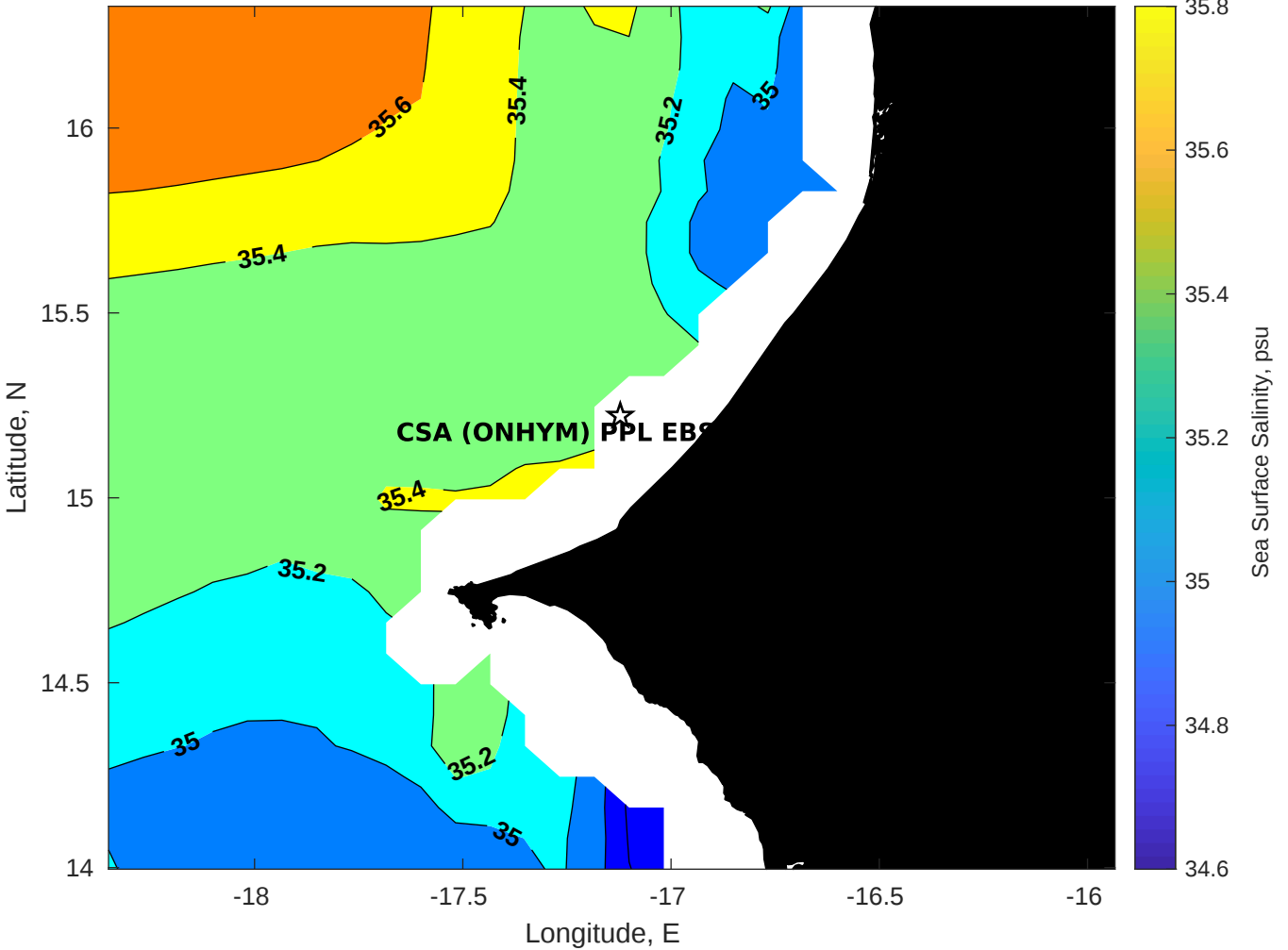
Surface Salinity for CSA (ONHYM) PPL EBS - Senegal at 20-Oct-2025 00:00:00
