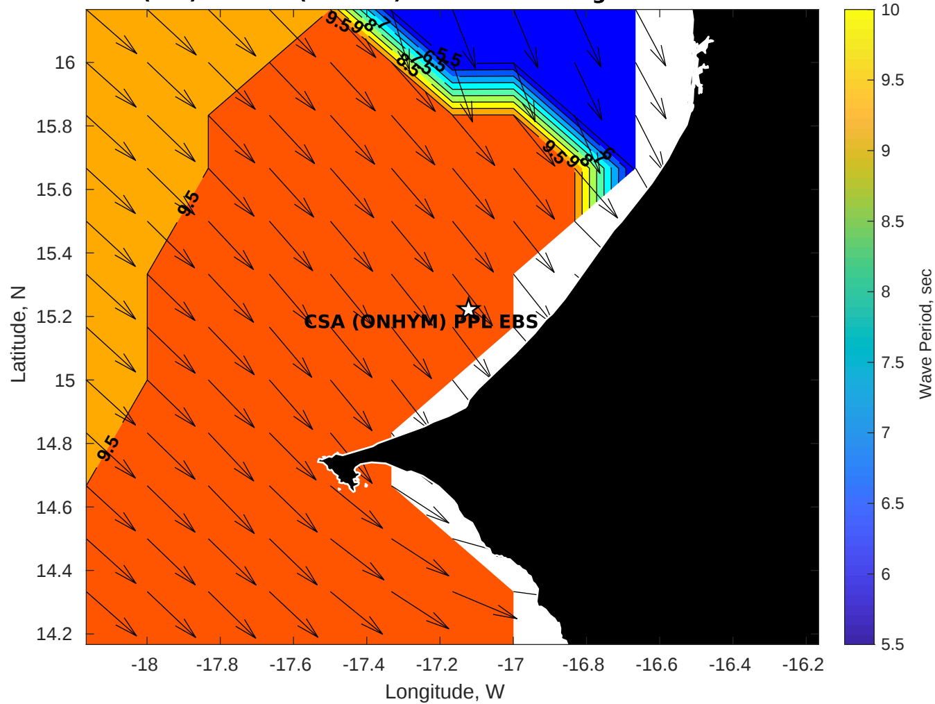
Wave Period (sec) for CSA (ONHYM) PPL EBS - Senegal at 21-Oct-2025 09:00:00
