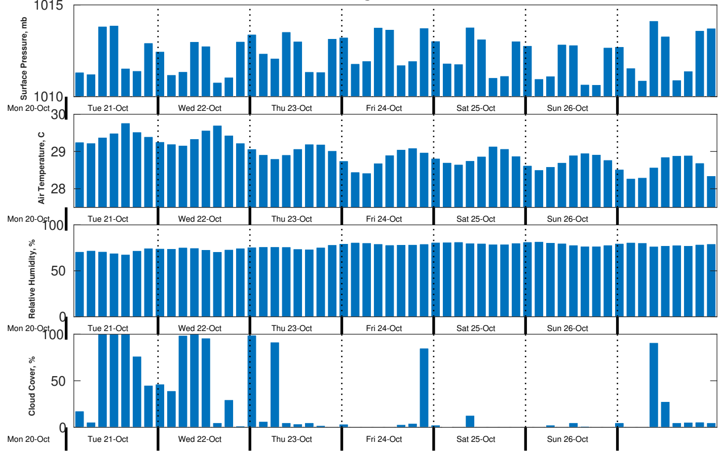
Met Forecast for CSA (ONHYM) PPL EBS - Senegal from 21-Oct-2025 00:00:00 to 28-Oct-2025 00:00:00
