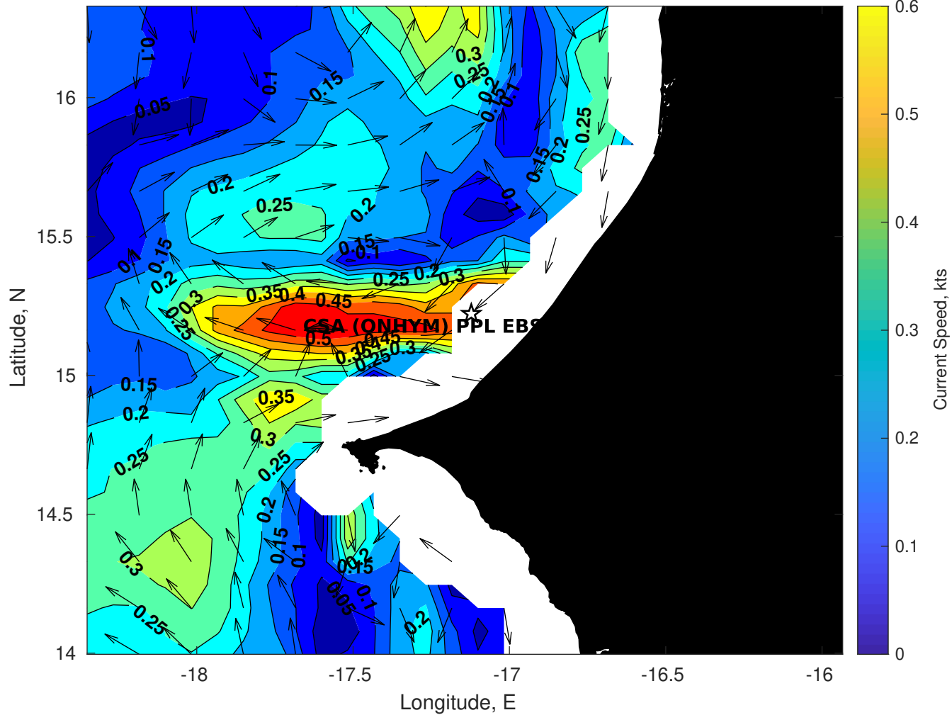
Surface Currents for CSA (ONHYM) PPL EBS - Senegal at 20-Oct-2025 00:00:00
