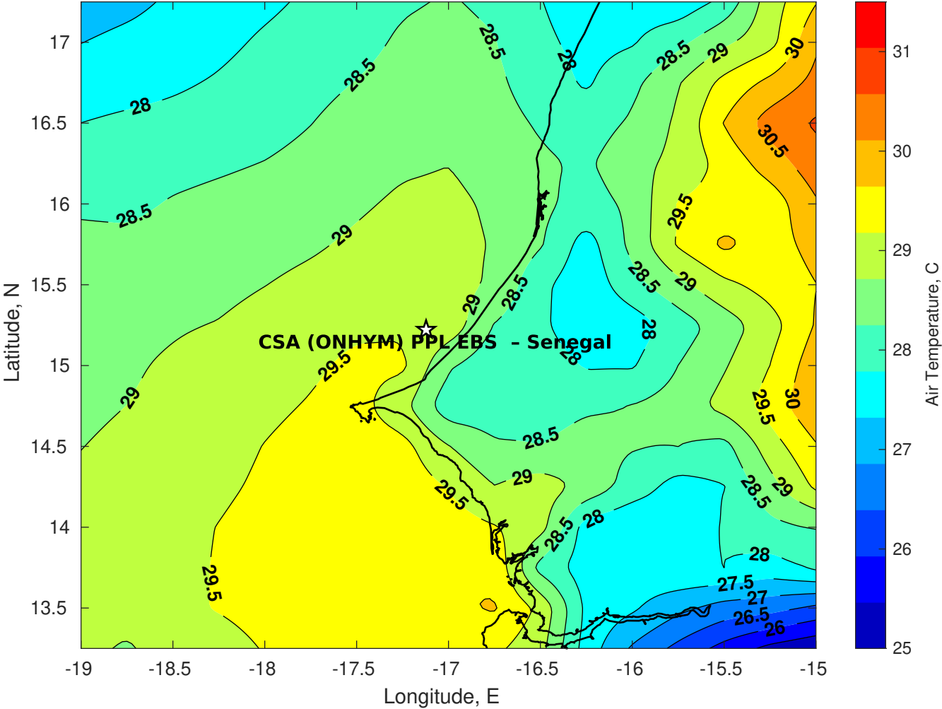
Air Temperature (C) for CSA (ONHYM) PPL EBS - Senegal at 21-Oct-2025
