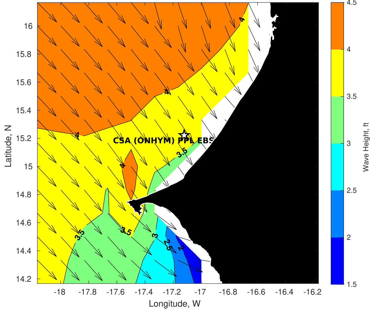
Wave Height (ft) for CSA (ONHYM) PPL EBS - Senegal at 21-Oct-2025 09:00:00
