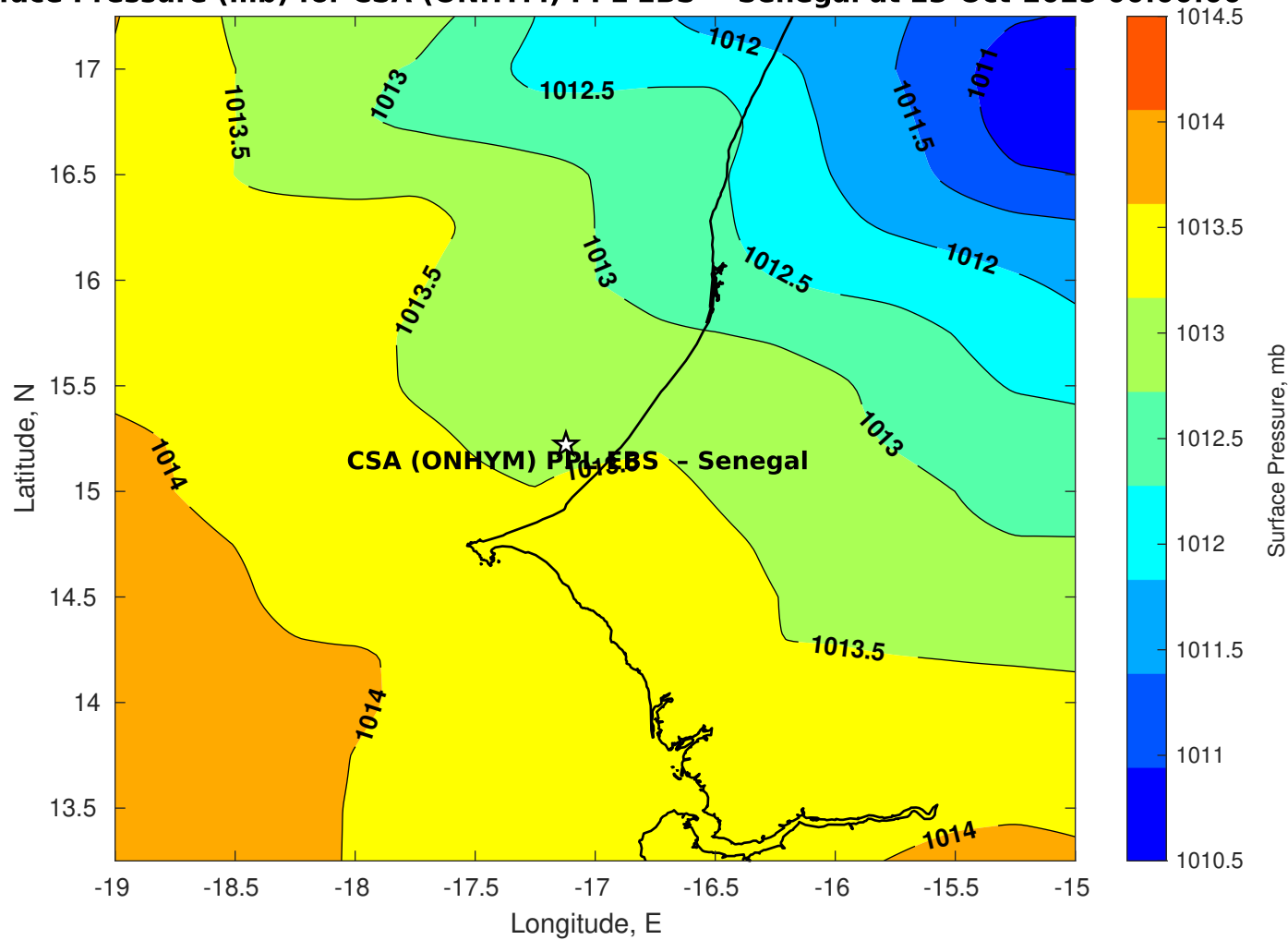
Surface Pressure (mb) for CSA (ONHYM) PPL EBS - Senegal at 23-Oct-2025 00:00:00
