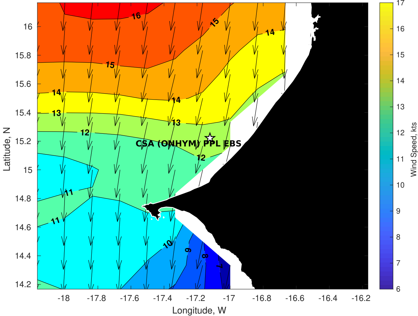
Winds (kts) for CSA (ONHYM) PPL EBS - Senegal at 21-Oct-2025 09:00:00
