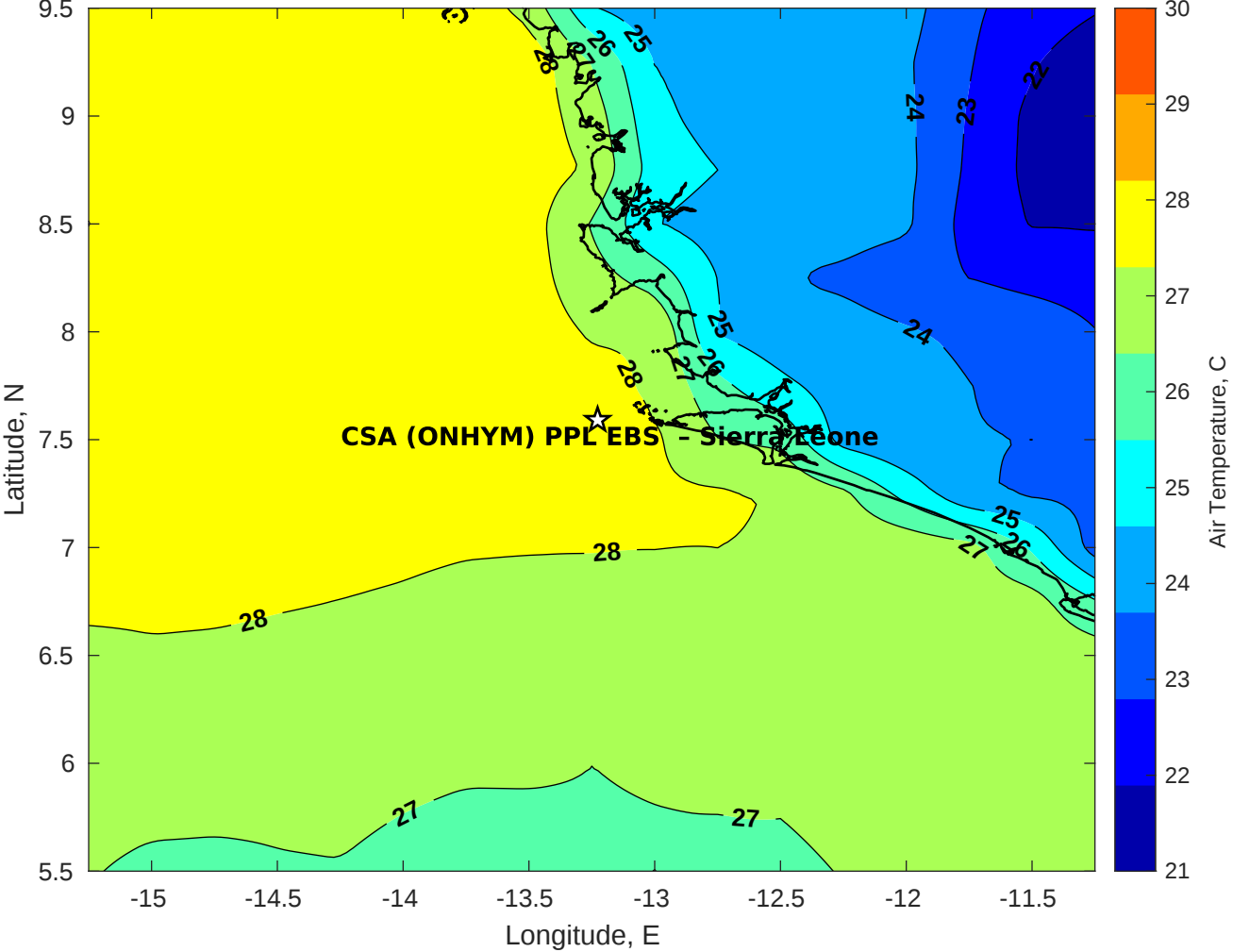
Air Temperature (C) for CSA (ONHYM) PPL EBS - Sierra Leone at 21-Oct-2025
