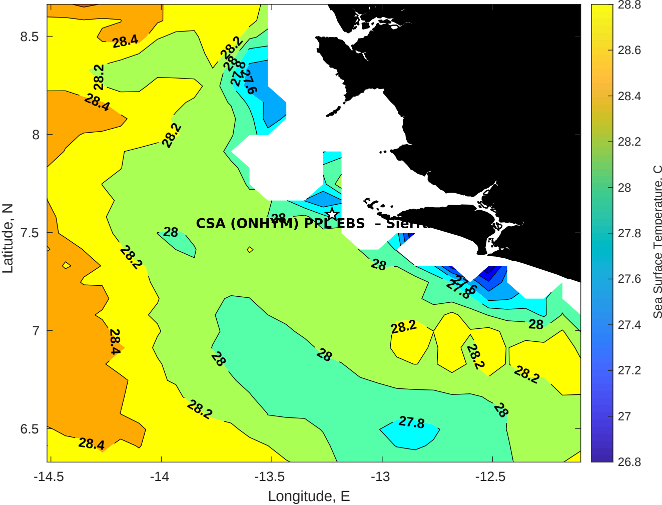
SST for CSA (ONHYM) PPL EBS - Sierra Leone at 20-Oct-2025 00:00:00
