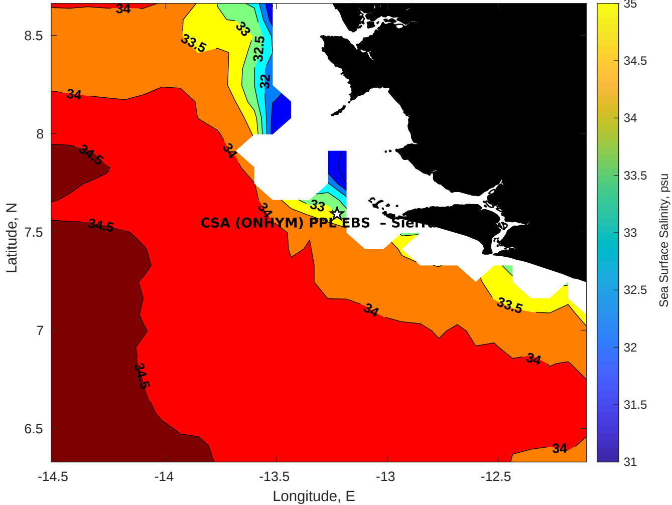
Surface Salinity for CSA (ONHYM) PPL EBS - Sierra Leone at 20-Oct-2025 00:00:00
