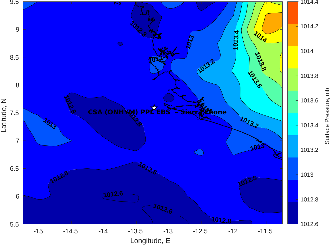
Surface Pressure (mb) for CSA (ONHYM) PPL EBS - Sierra Leone at 21-Oct-2025 00:00:00
