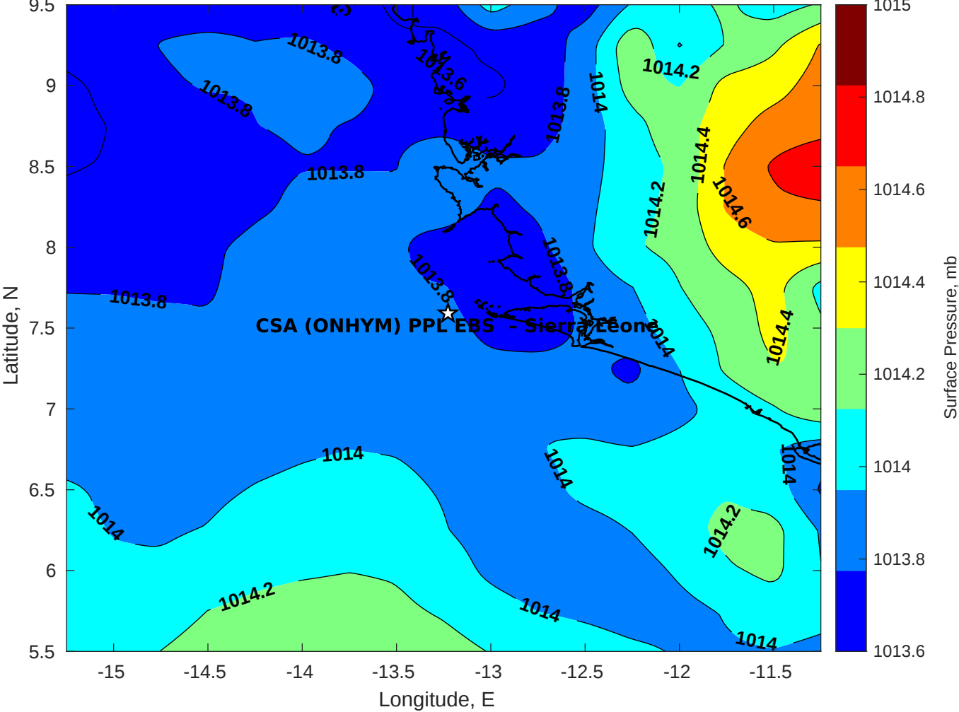
Surface Pressure (mb) for CSA (ONHYM) PPL EBS - Sierra Leone at 22-Oct-2025 00:00:00
