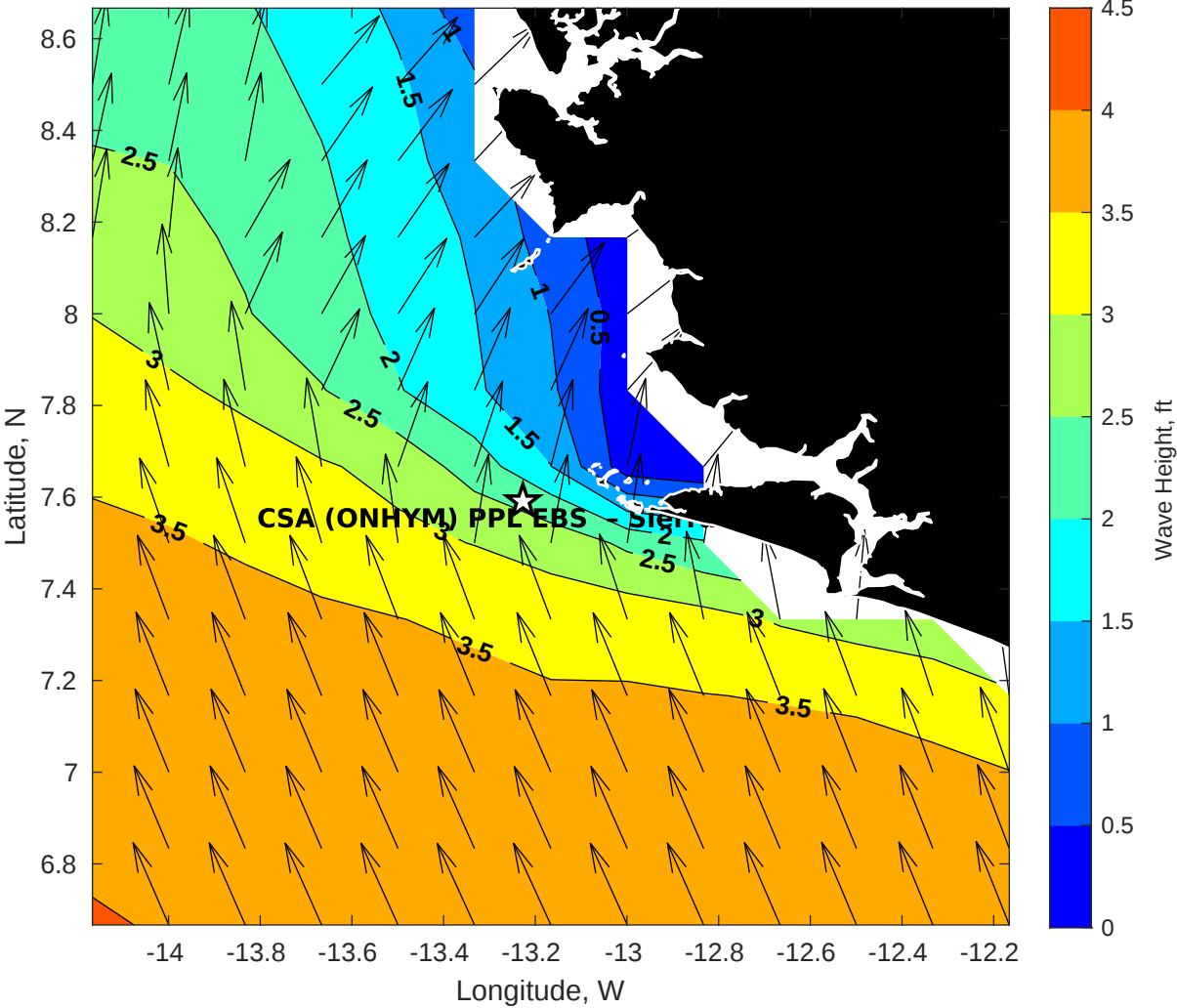
Wave Height (ft) for CSA (ONHYM) PPL EBS - Sierra Leone at 21-Oct-2025 09:00:00
