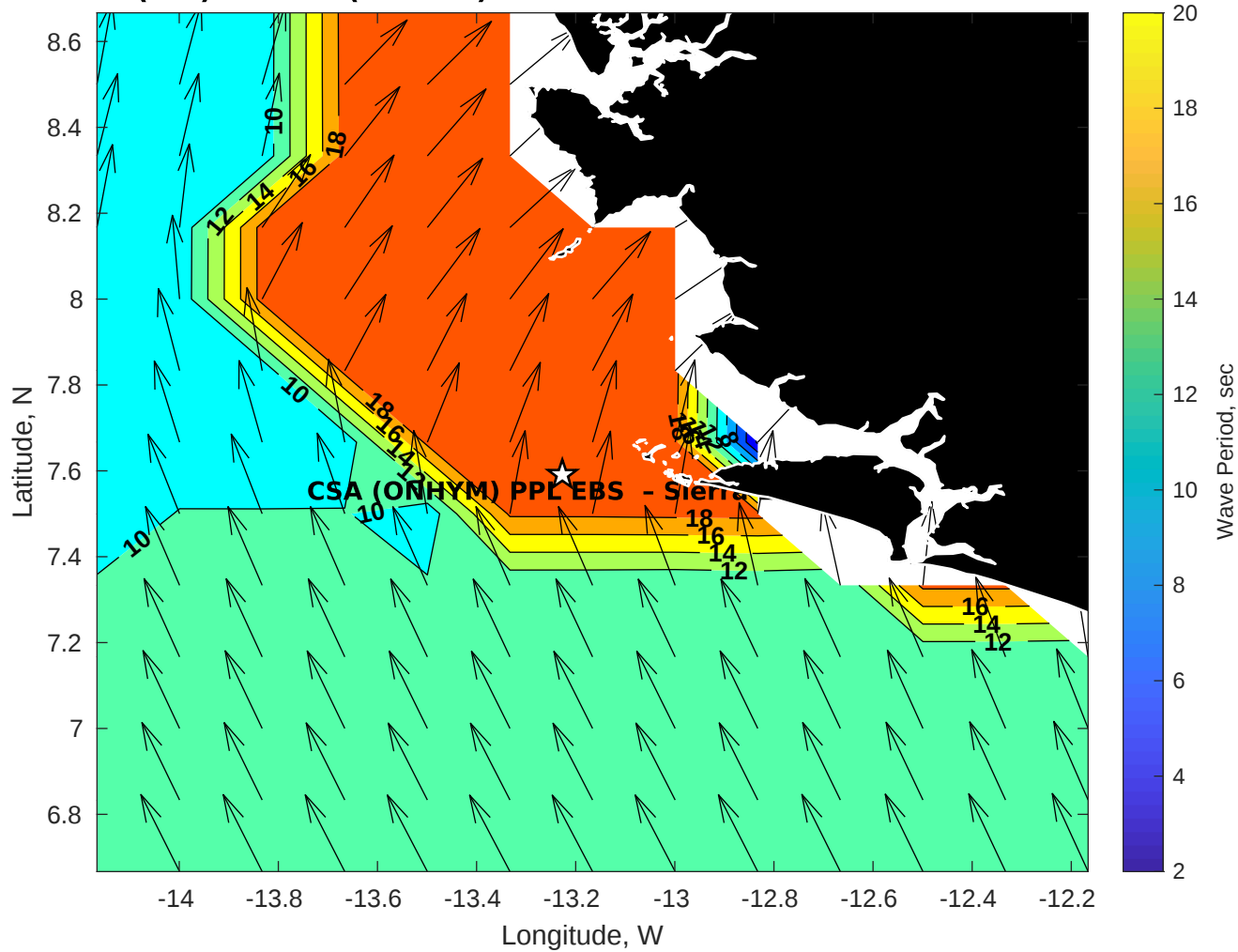
Wave Period (sec) for CSA (ONHYM) PPL EBS - Sierra Leone at 21-Oct-2025 09:00:00
