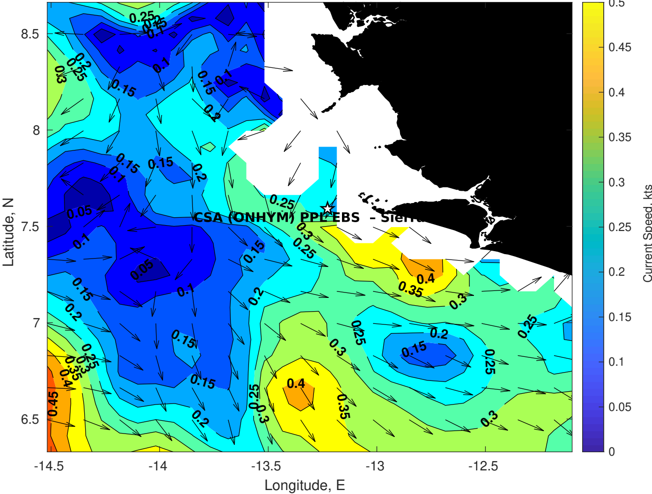
Surface Currents for CSA (ONHYM) PPL EBS - Sierra Leone at 20-Oct-2025 00:00:00
