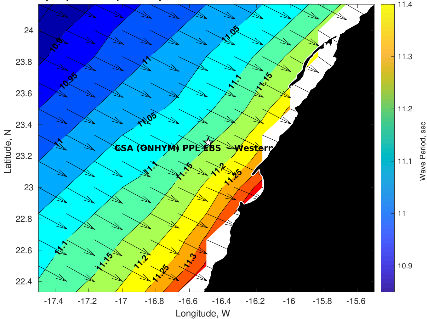
Wave Period (sec) for CSA (ONHYM) PPL EBS - Western Sahara at 21-Oct-2025 09:00:00
