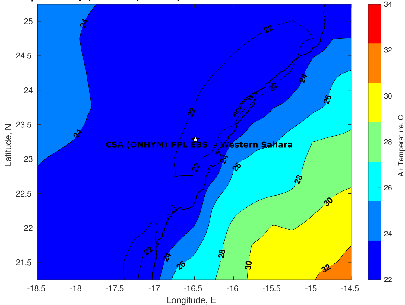
Air Temperature (C) for CSA (ONHYM) PPL EBS - Western Sahara at 21-Oct-2025
