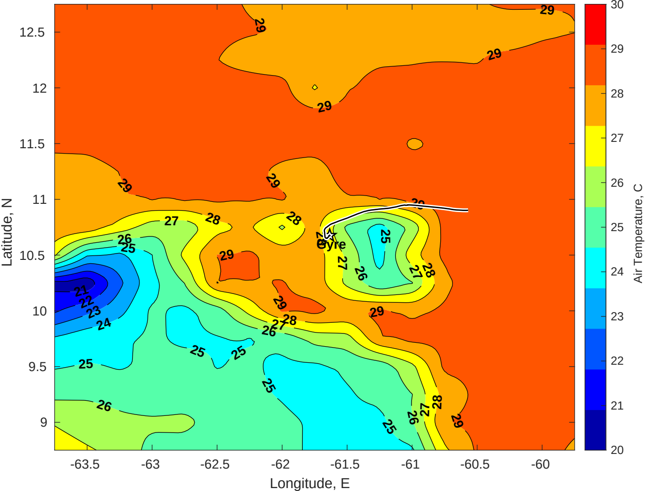
Air Temperature (C) for Gyre at 21-Oct-2025
