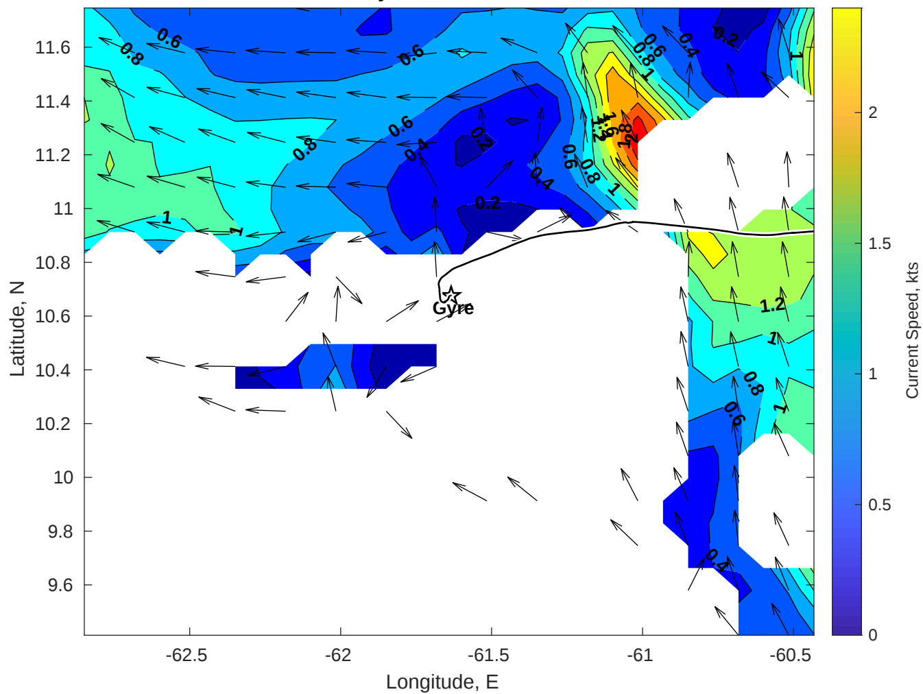
Surface Currents for Gyre at 20-Oct-2025 00:00:00
