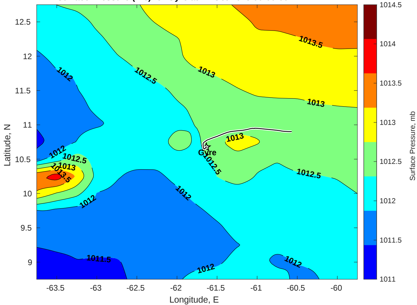
Surface Pressure (mb) for Gyre at 21-Oct-2025 00:00:00
