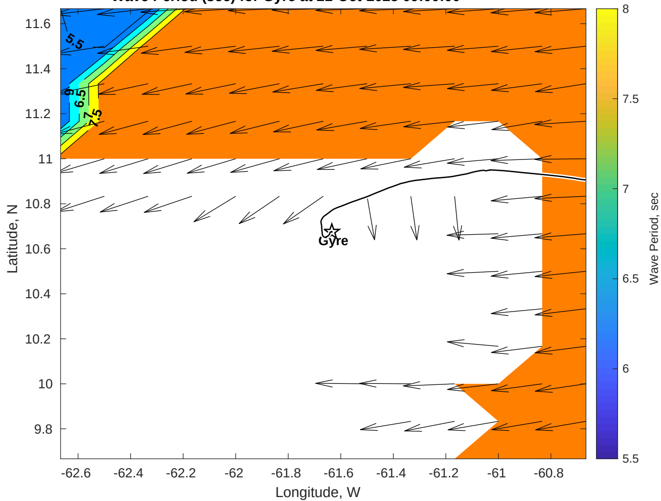
Wave Period (sec) for Gyre at 21-Oct-2025 09:00:00
