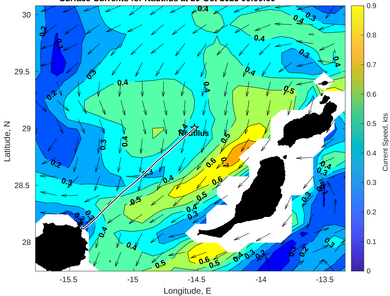
Surface Currents for Nautilus at 20-Oct-2025 00:00:00
