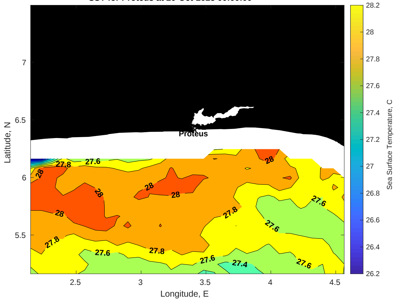
SST for Proteus at 20-Oct-2025 00:00:00
