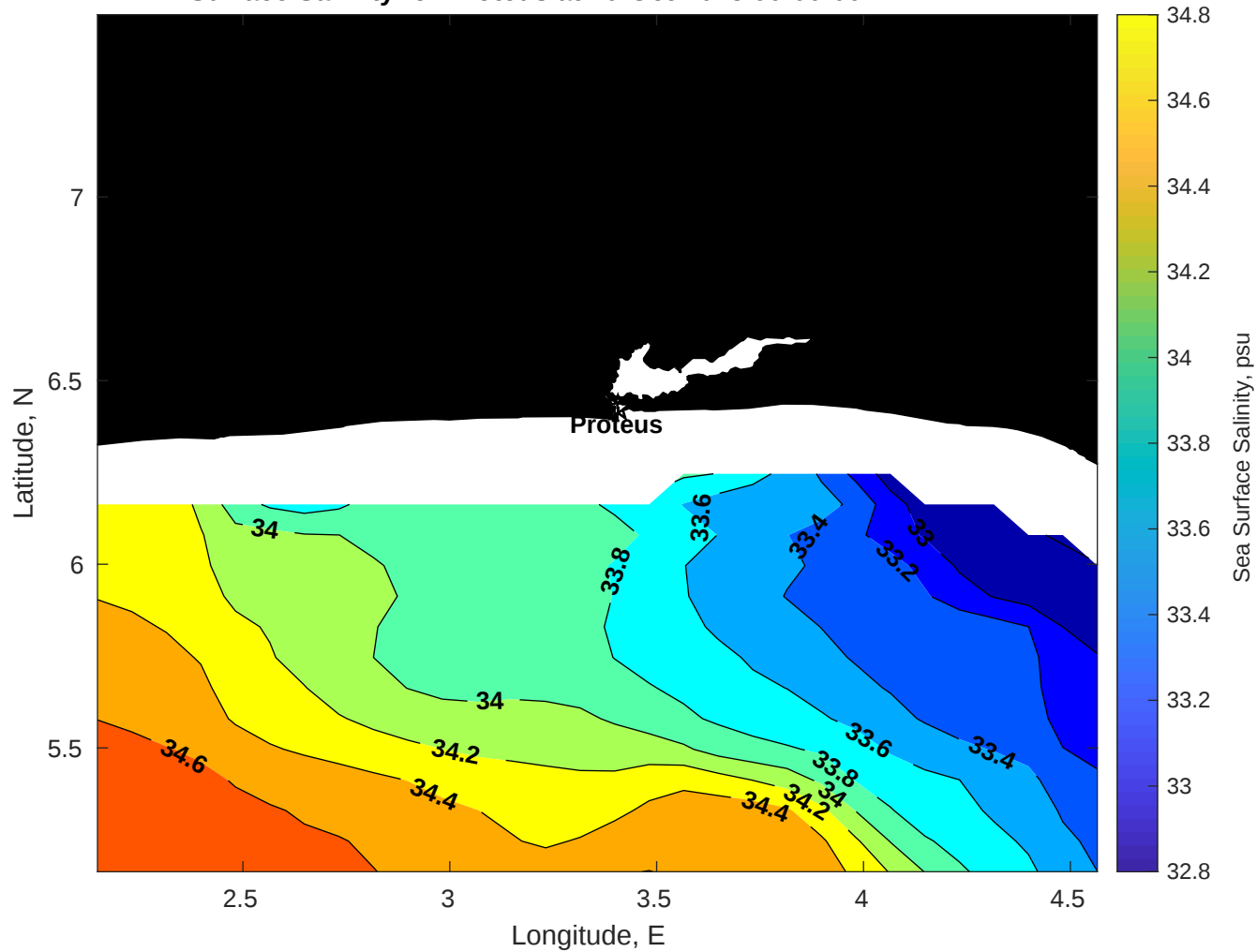
Surface Salinity for Proteus at 20-Oct-2025 00:00:00
