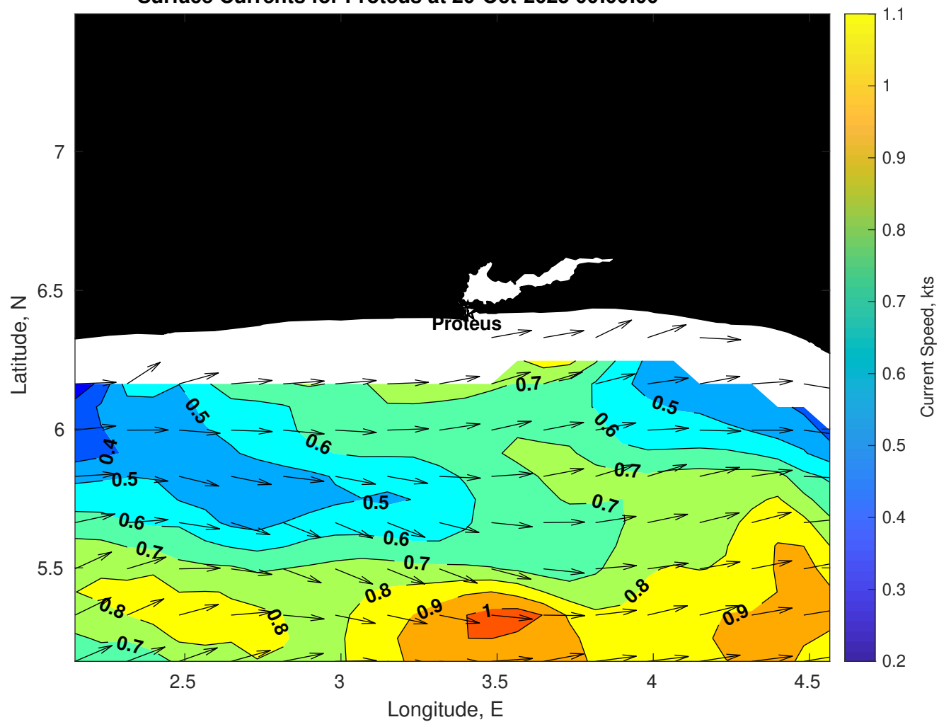
Surface Currents for Proteus at 20-Oct-2025 00:00:00
