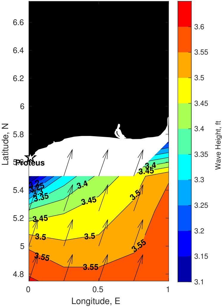
Wave Height (ft) for Proteus at 21-Oct-2025 09:00:00
