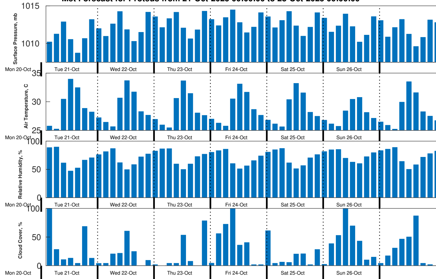
Met Forecast for Proteus from 21-Oct-2025 00:00:00 to 28-Oct-2025 00:00:00
