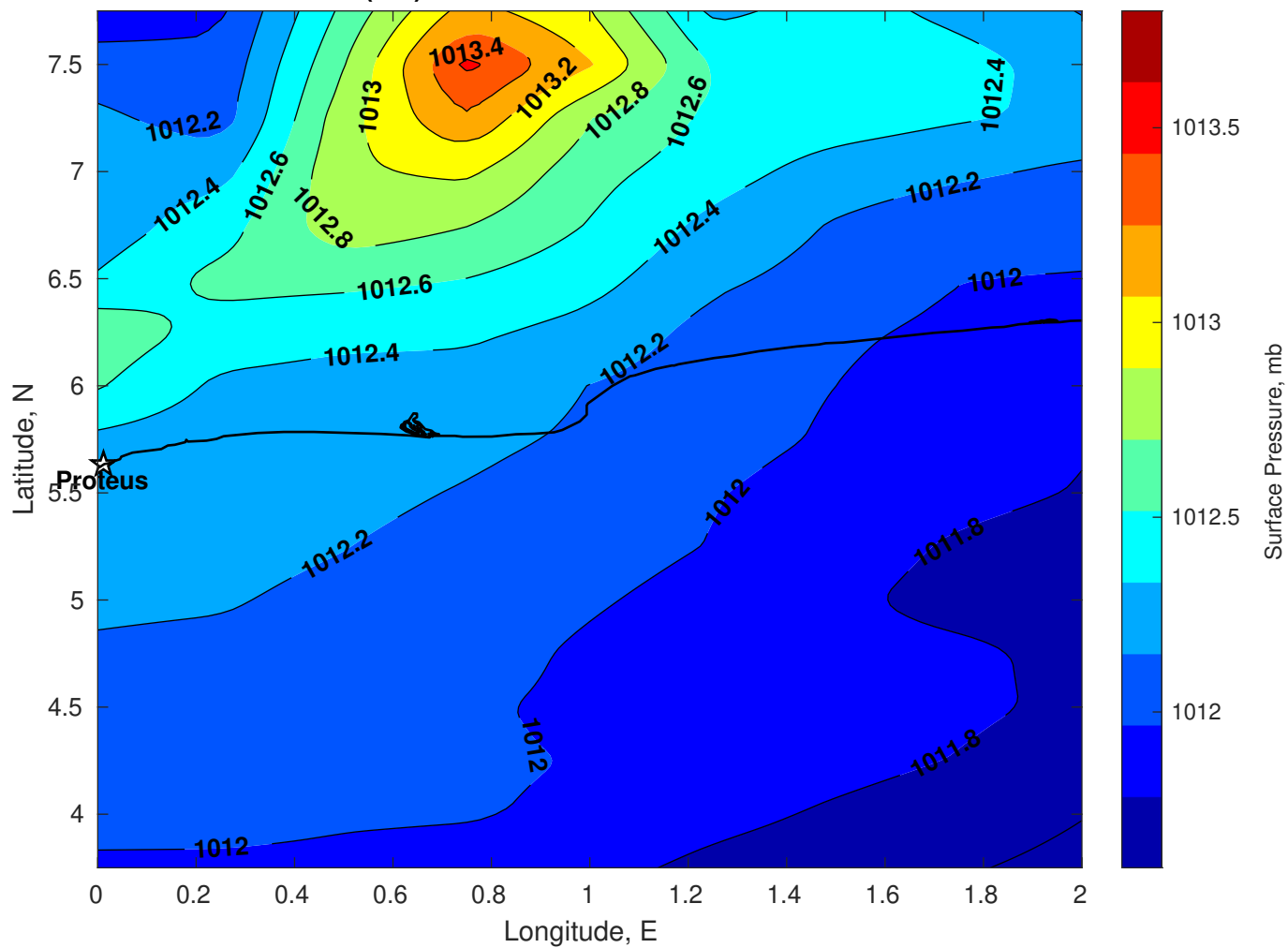
Surface Pressure (mb) for Proteus at 21-Oct-2025 00:00:00
