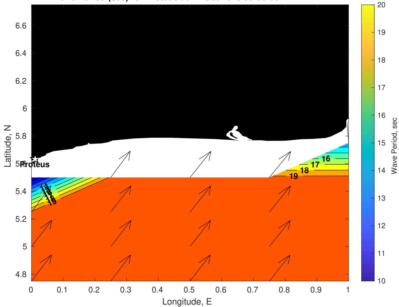
Wave Period (sec) for Proteus at 21-Oct-2025 09:00:00
