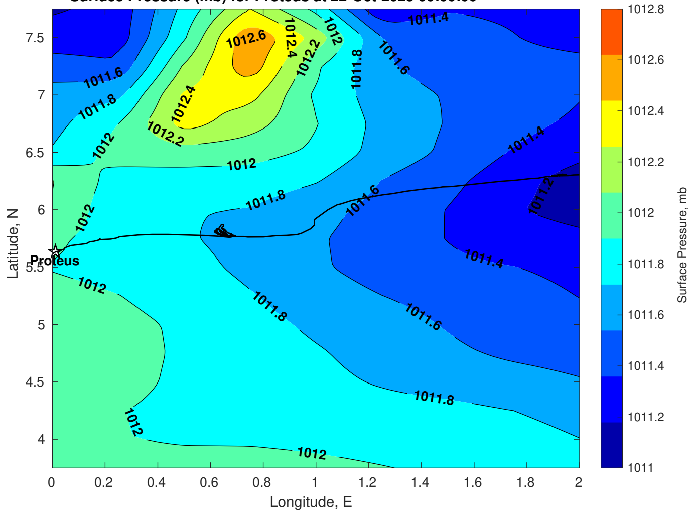
Surface Pressure (mb) for Proteus at 22-Oct-2025 00:00:00
