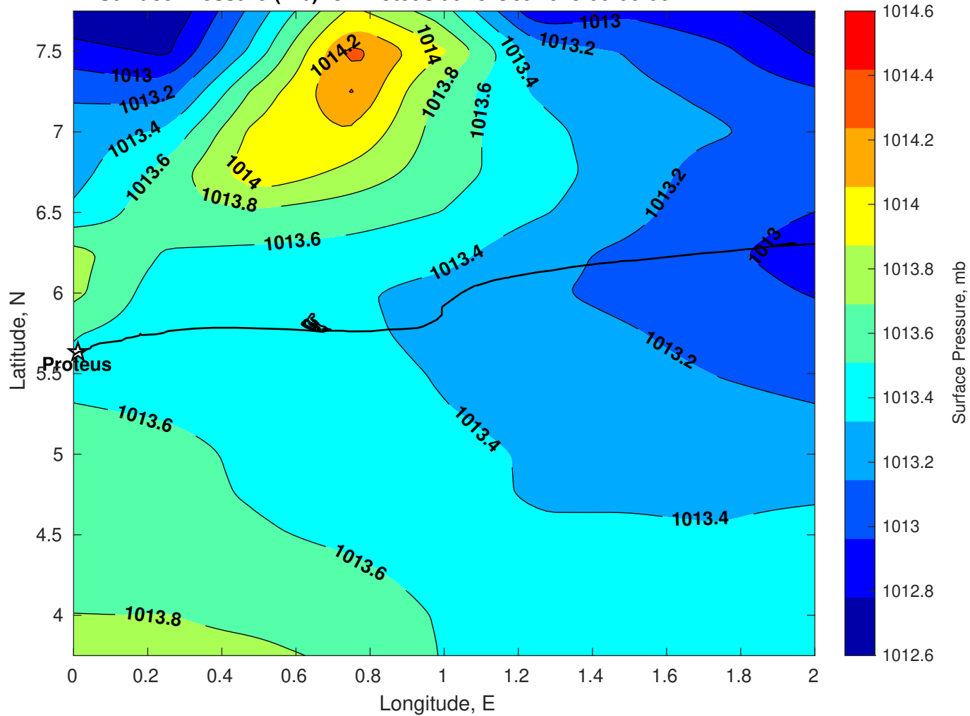
Surface Pressure (mb) for Proteus at 23-Oct-2025 00:00:00
