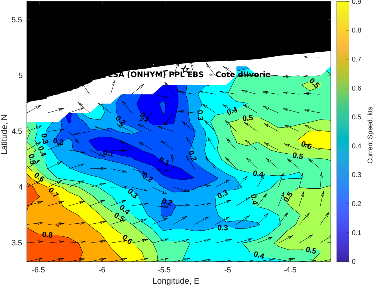
Surface Currents for CSA (ONHYM) PPL EBS - Cote d'Ivoire at 21-Oct-2025 00:00:00
