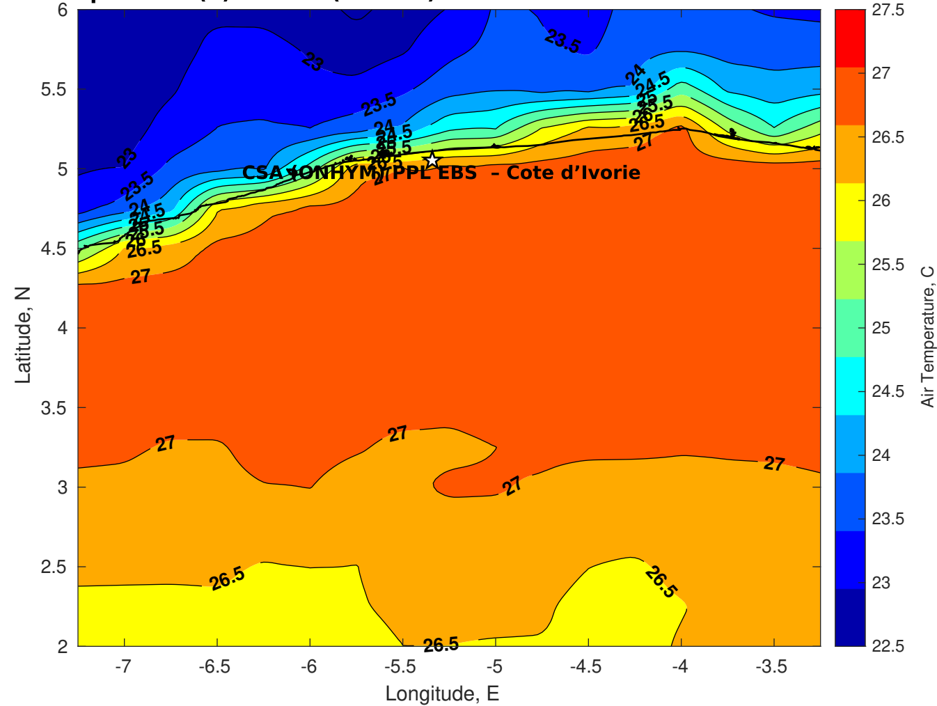
Air Temperature (C) for CSA (ONHYM) PPL EBS - Cote d'Ivoire at 22-Oct-2025
