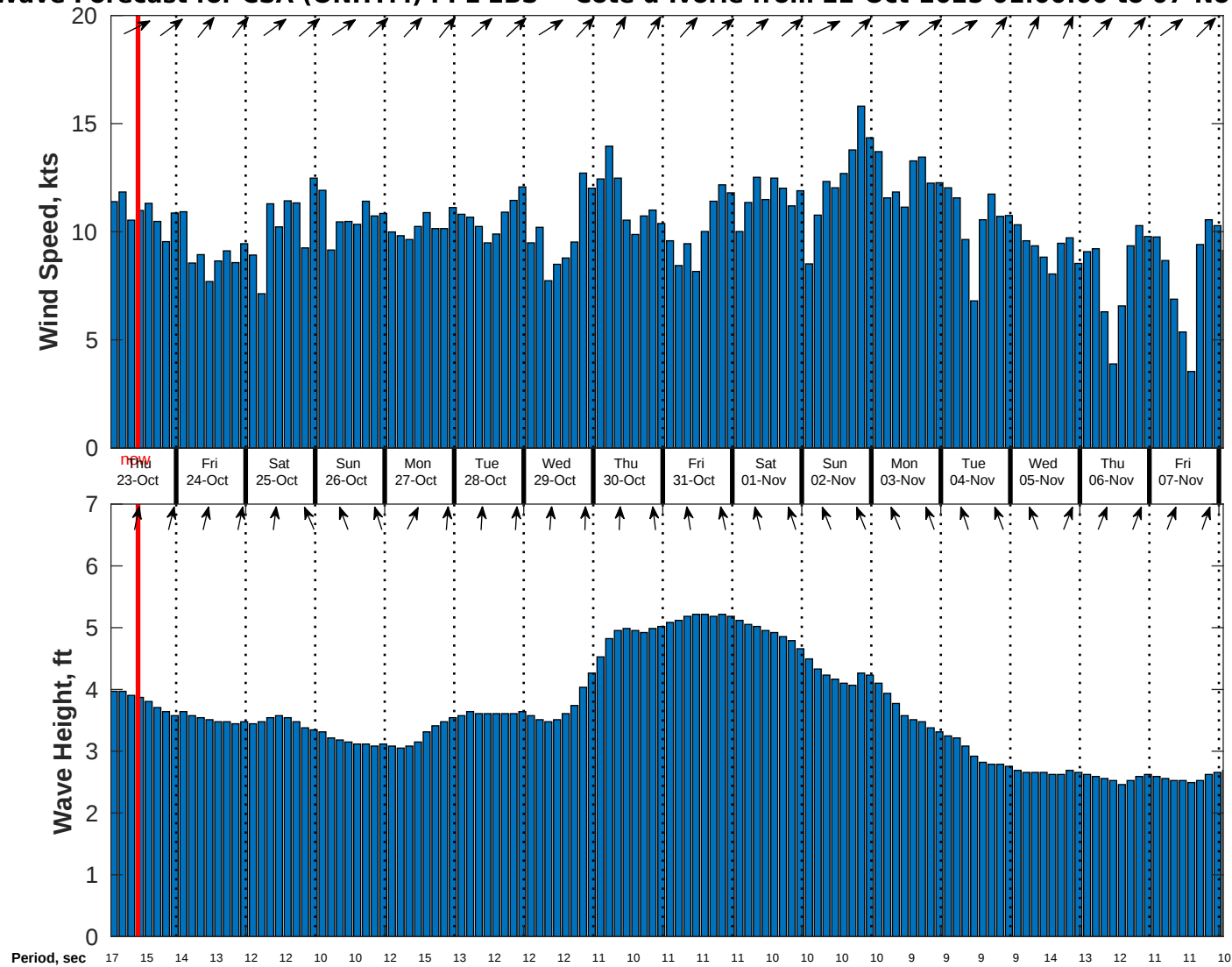
Wind & Wave Forecast for CSA (ONHYM) PPL EBS - Cote d'Ivoire from 22-Oct-2025 01:00:00 to 07-Nov-2025 01:00:00
