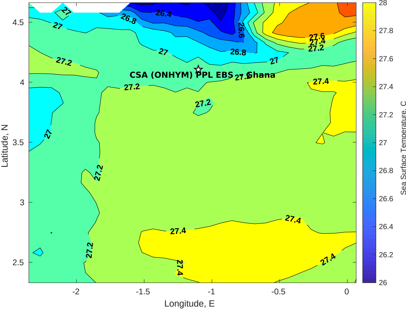
SST for CSA (ONHYM) PPL EBS - Ghana at 21-Oct-2025 00:00:00
