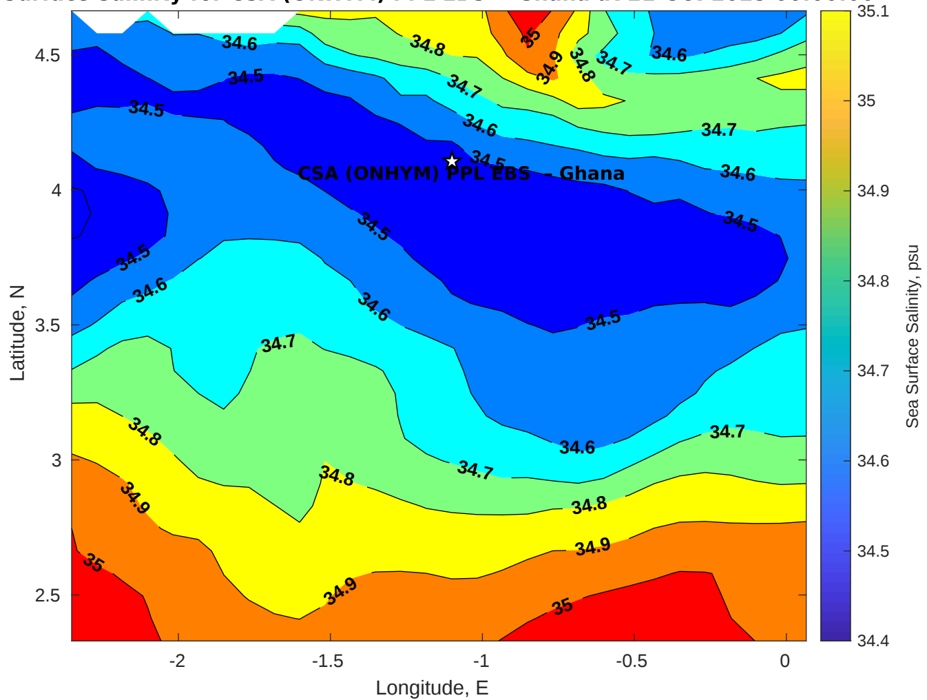
Surface Salinity for CSA (ONHYM) PPL EBS - Ghana at 21-Oct-2025 00:00:00
