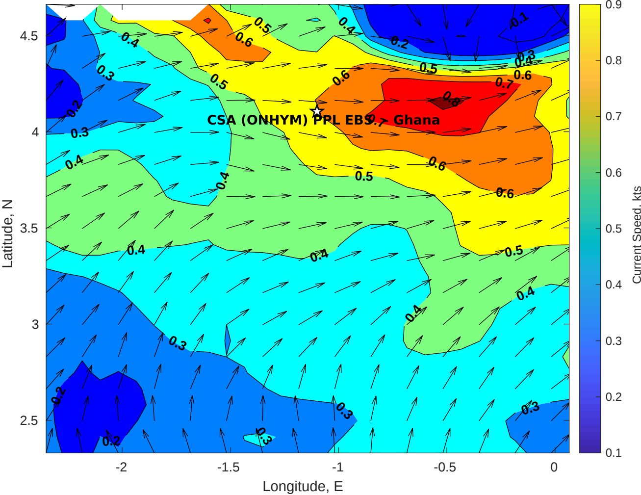
Surface Currents for CSA (ONHYM) PPL EBS - Ghana at 21-Oct-2025 00:00:00
