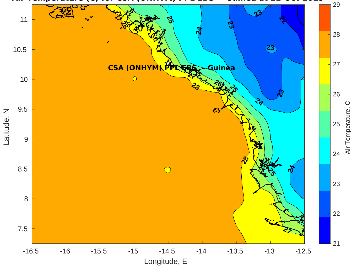
Air Temperature (C) for CSA (ONHYM) PPL EBS - Guinea at 22-Oct-2025
