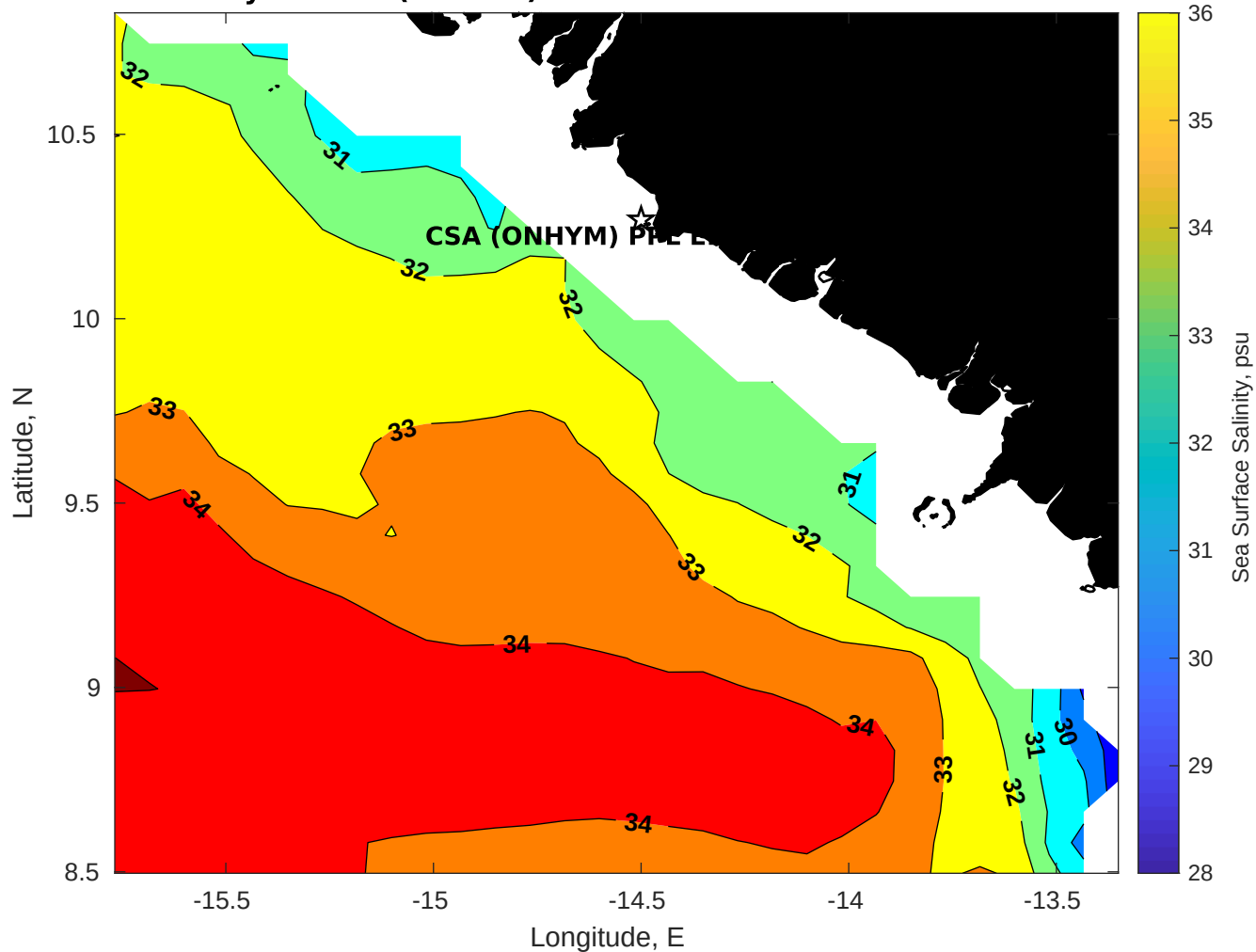
Surface Salinity for CSA (ONHYM) PPL EBS - Guinea at 21-Oct-2025 00:00:00
