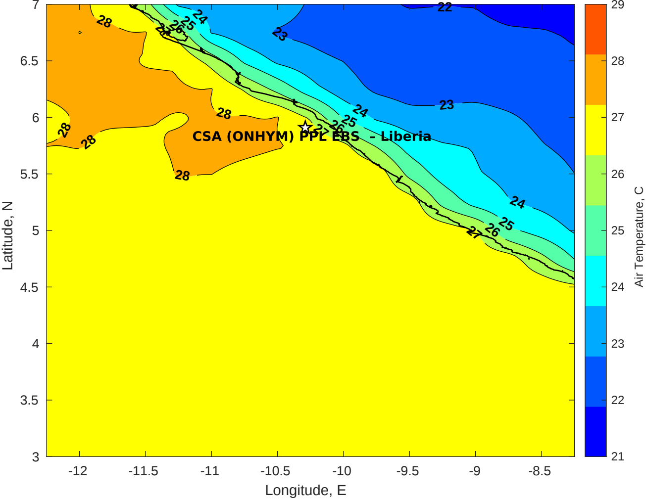
Air Temperature (C) for CSA (ONHYM) PPL EBS - Liberia at 22-Oct-2025
