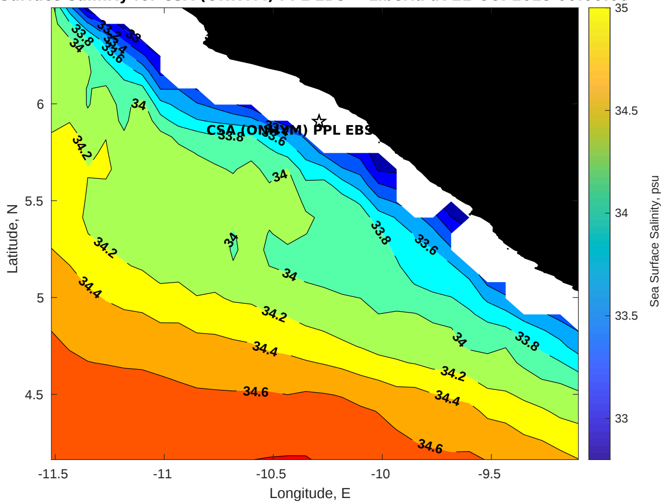
Surface Salinity for CSA (ONHYM) PPL EBS - Liberia at 21-Oct-2025 00:00:00
