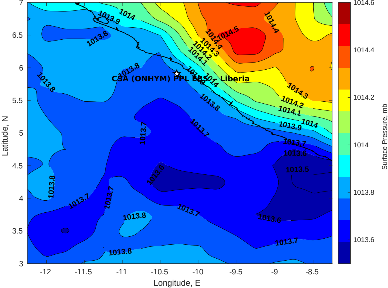
Surface Pressure (mb) for CSA (ONHYM) PPL EBS - Liberia at 22-Oct-2025 00:00:00
