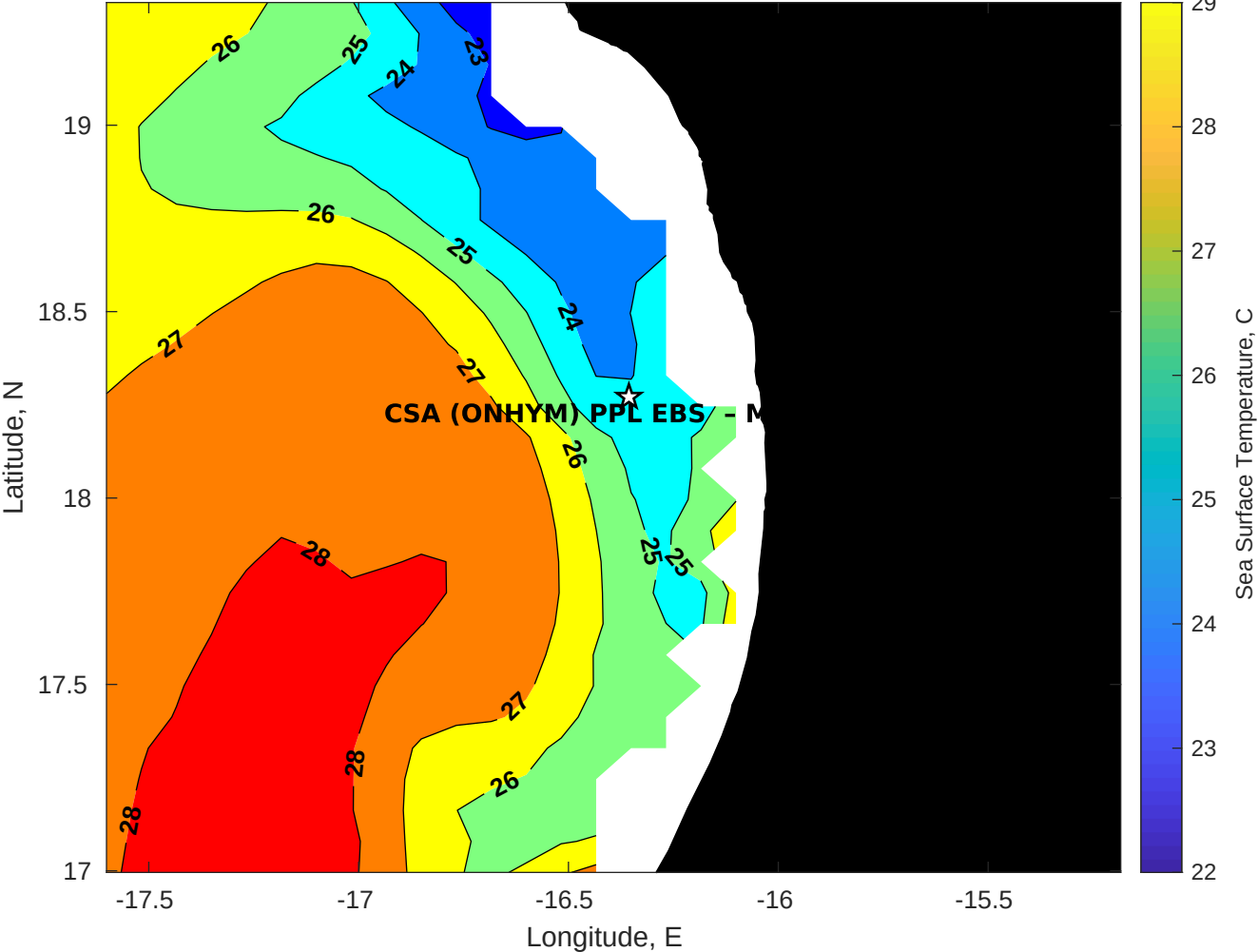
SST for CSA (ONHYM) PPL EBS - Mauritania at 21-Oct-2025 00:00:00
