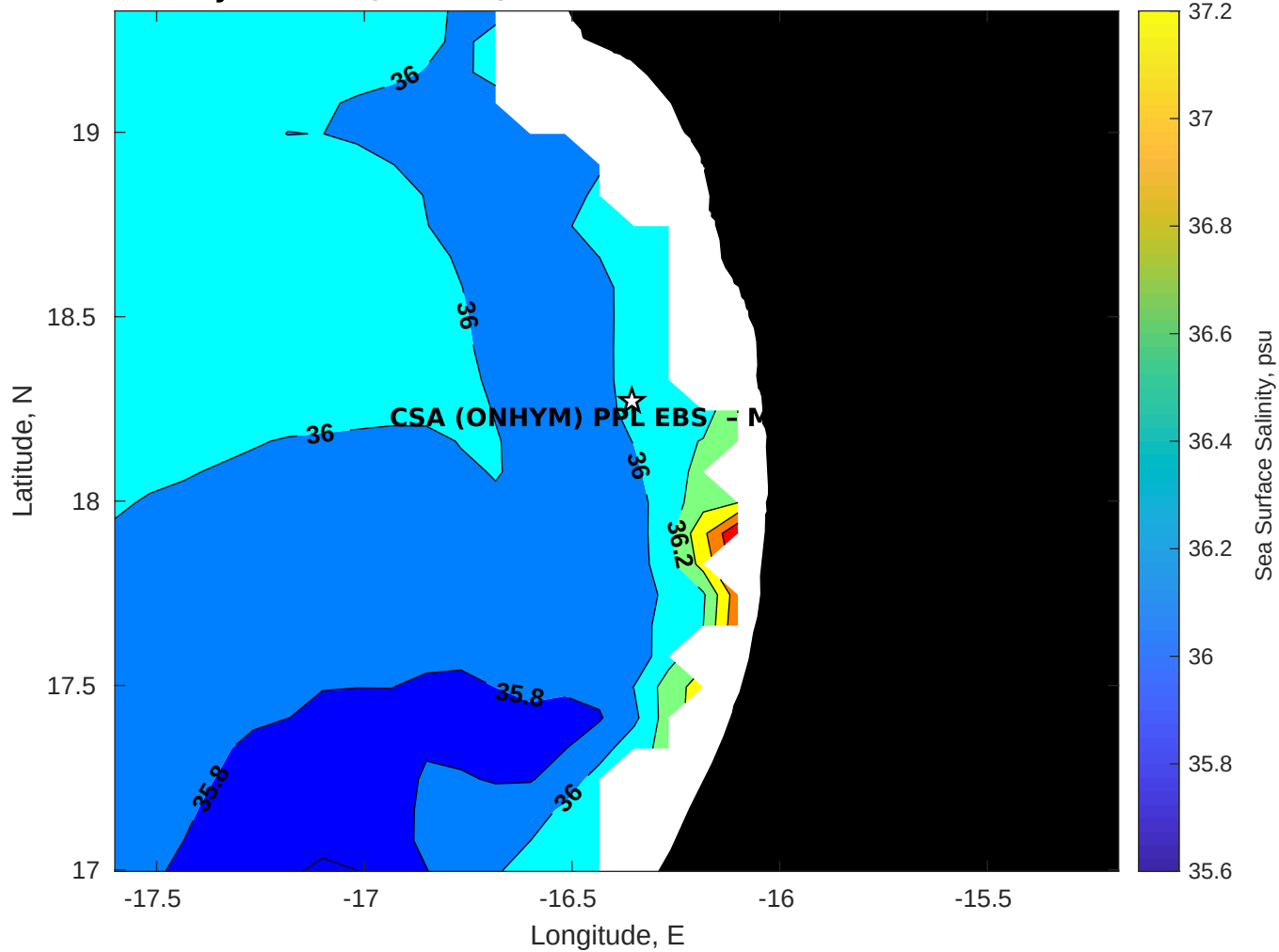
Surface Salinity for CSA (ONHYM) PPL EBS - Mauritania at 21-Oct-2025 00:00:00
